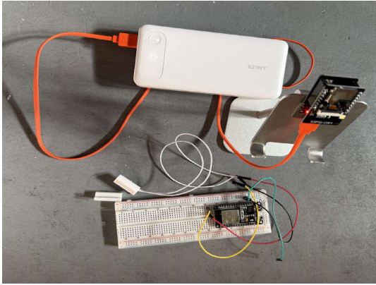
Figure 8.1.1 Main System Prototype (Left), Servo System Prototype (Right)
