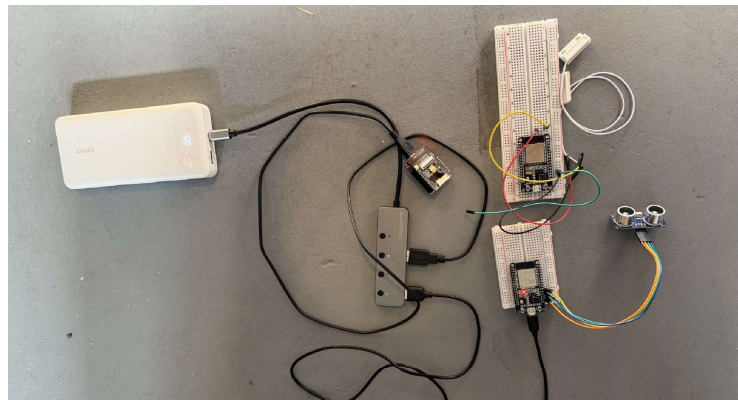
Figure 8.1.2 Object Detection System Prototype
