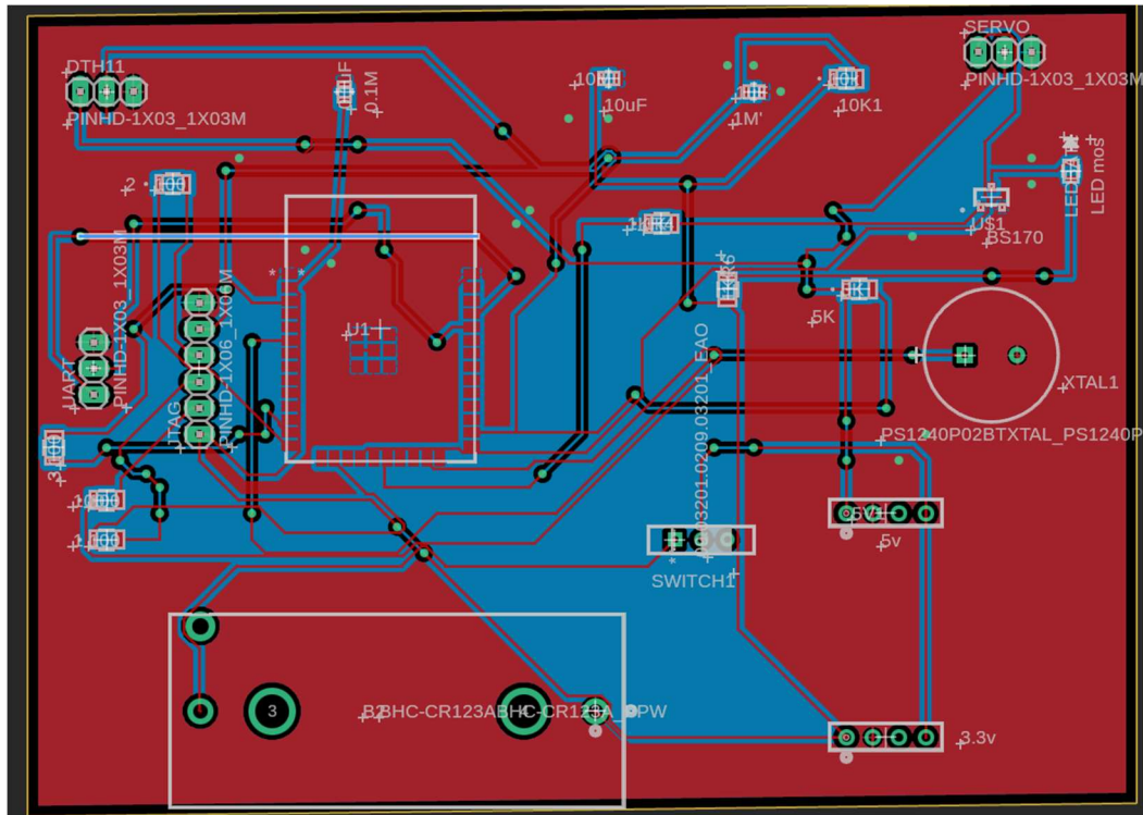
Figure 8.2.1 Servo system PCB layout
