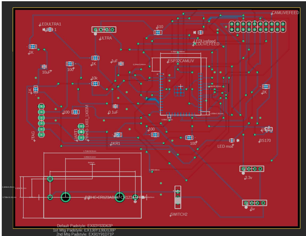
Figure 8.2.3 Live feed camera system PCB layout
