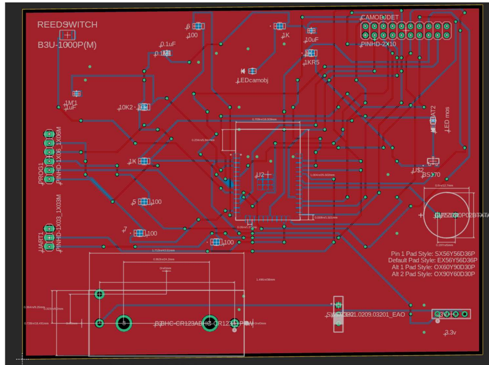
Figure 8.2.2 Object Detection Camera System PCB layout
