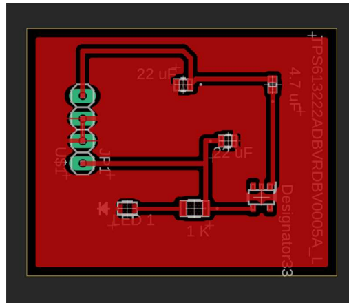
Figure 8.2.4 3.3V and 5V Voltage Regulator PCB layout
