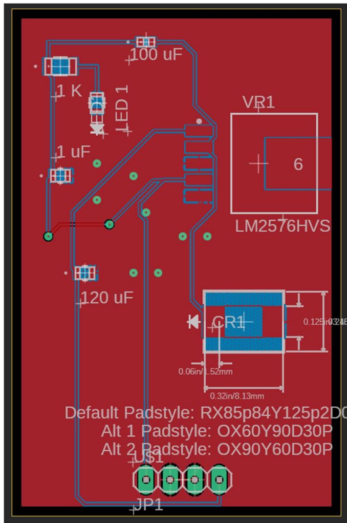
8.2.6 LM2576 5V buck regulator PCB
