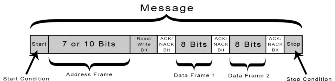
Figure 3.1.6.3.2 I2C Frame
