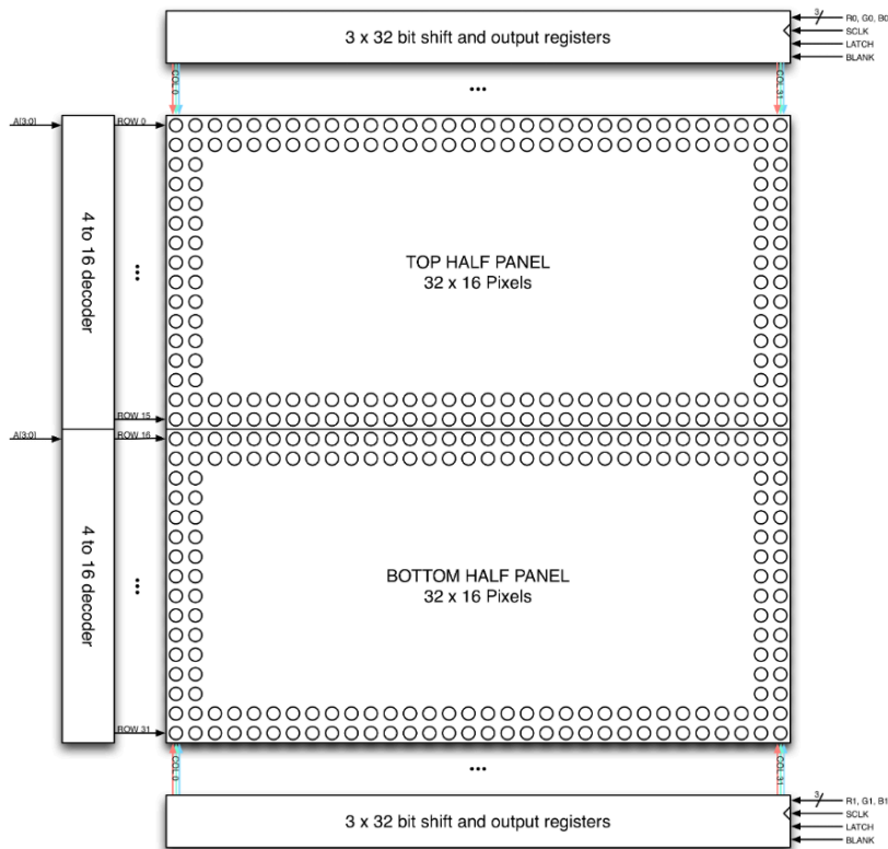
Image 2.9.3: 32x32 LED Matrix
