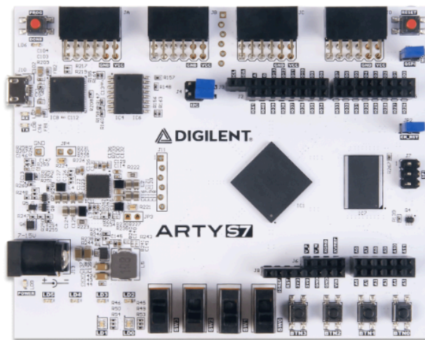
Image 2.9.1: Arty S7-50: Spartan-7 FPGA
