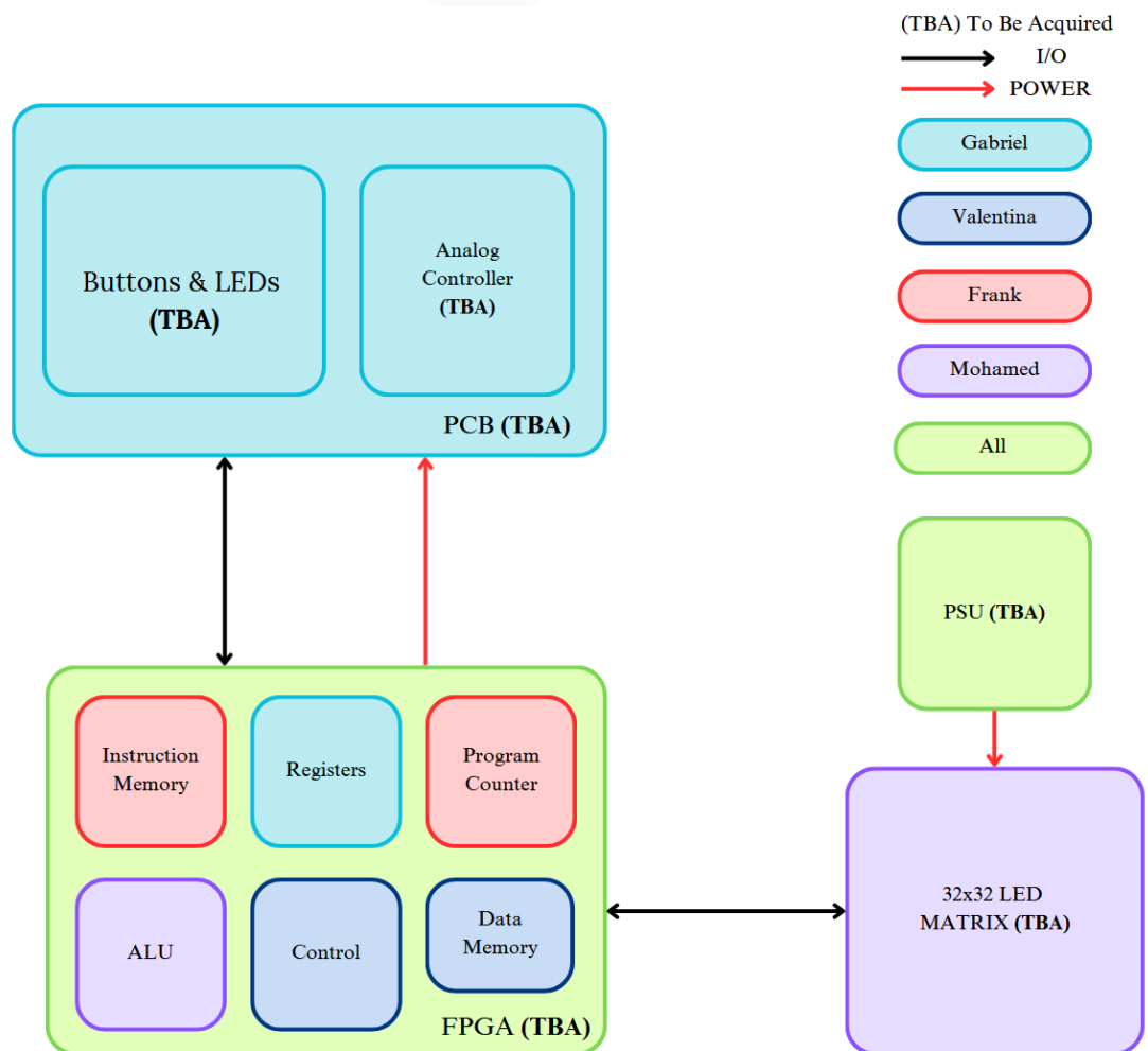
Figure 2.1: Hardware Overview
