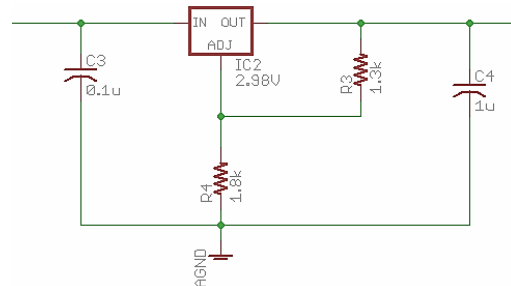
Figure 36: LM317-ADJ setup for a 2.98V
