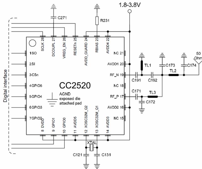
Figure 45: Reference design for the CC2520 Reprinted with permission from Ti.com
