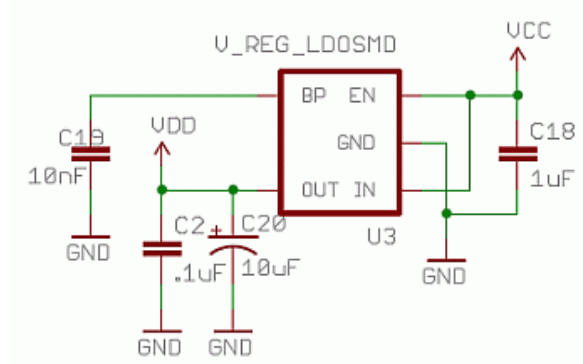
Figure 22: Power regulation for the IDG-500 gyro Reprinted with permission from Sparkfun.
