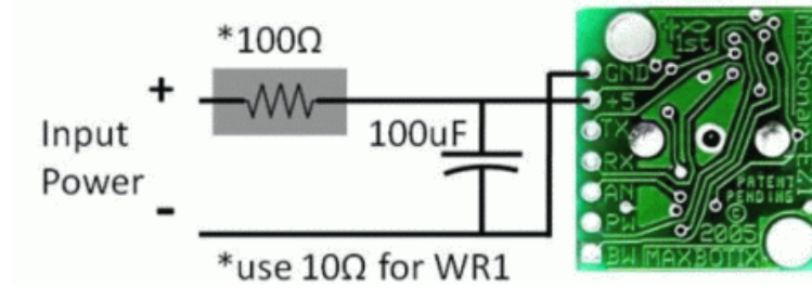
Figure 27: MaxBotix recommended low-pass filter. Reprinted with permission from MaxBotix
