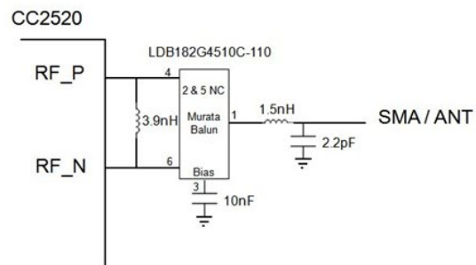
Figure 16: Balun circuit for the CC2520 Reprinted with permission from TI.com
