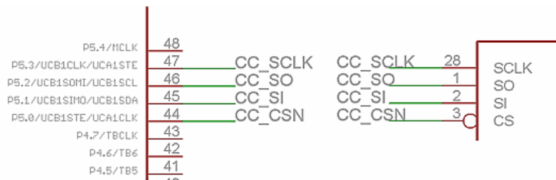
Figure 46: Schematic of SPI MSP430F2616 and the CC2520
