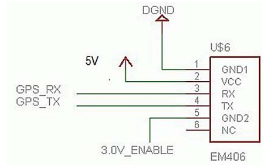
Figure 44: EM406 connector for the MT3329 GPS module
