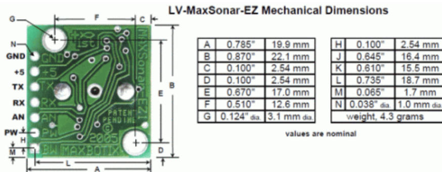
Figure 26: LV-MaxSonar-EZ Mechanical dimensions Reprinted with permission from MaxBotix Inc.
