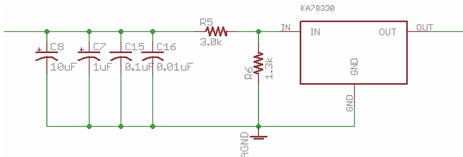
Figure 38: Voltage Detector Design Using the KA75330
