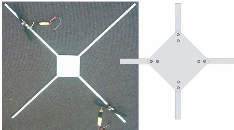
Figure 49: Aluminum prototype frame with close-up of central plate
