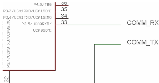
Figure 48: UART from MSP430F2616 to ATmega2560
