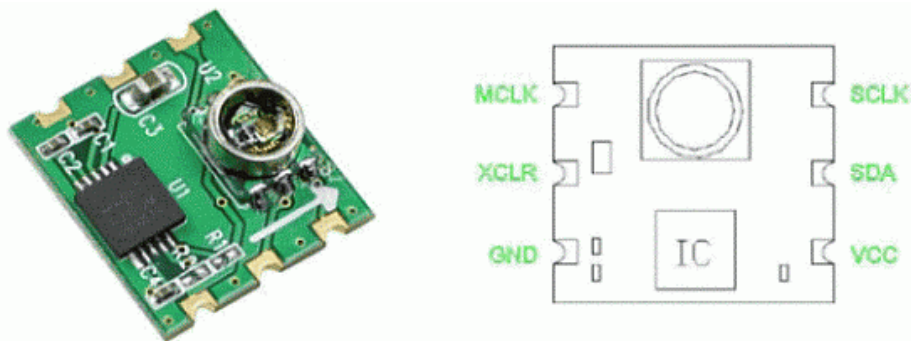
Figure 10: Hoperf electronics' HDPM01 pressure sensor and digital compass Reprinted with permission from Futurlec.com.
