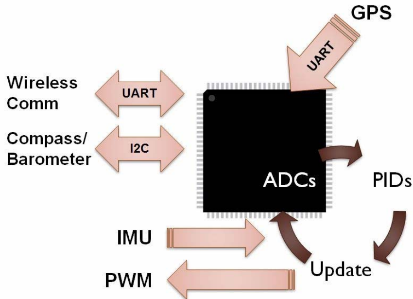
Figure 39: Overview of MCU interfaces
