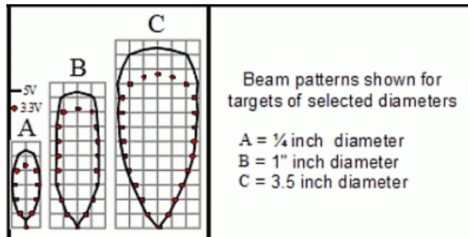
Figure 28: LV-MaxSonar-ez1 beam pattern diagram. Reprinted with permission from MaxBotix.
