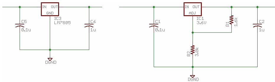
Figure 37: LM7805 and the LM317-ADJ at 3.6V
