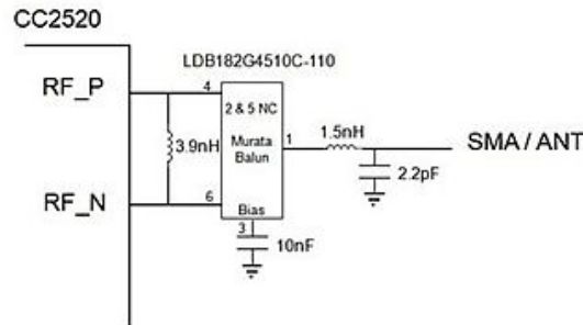
Figure 47: Balun circuit for the CC2520 Reprinted with permission from TI.com
