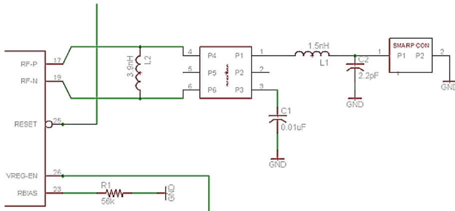
Figure 52: Radio Frequency Circuitry.
