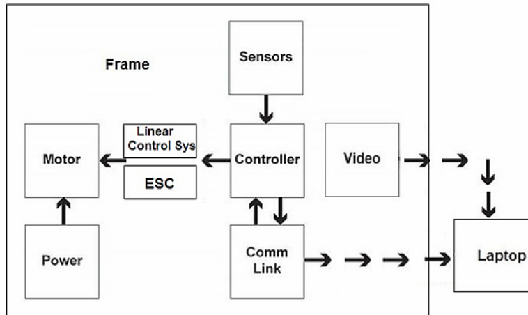
Figure 35: block diagram of quad-copter subsystems
