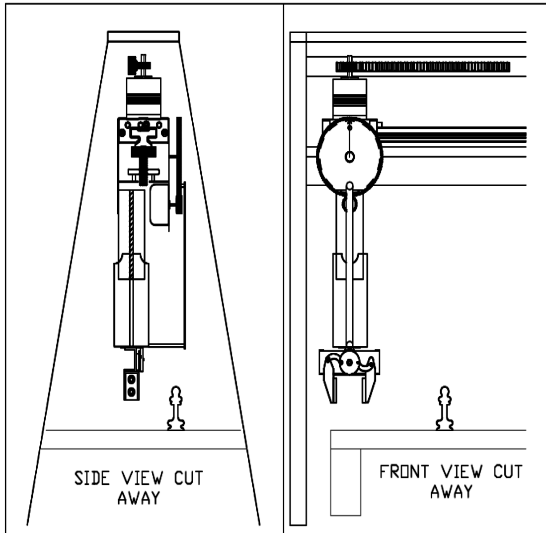
Figure 3.8-1: Grabber and Z axis cut away views. This picture was drawn using AutoCAD educational software.
