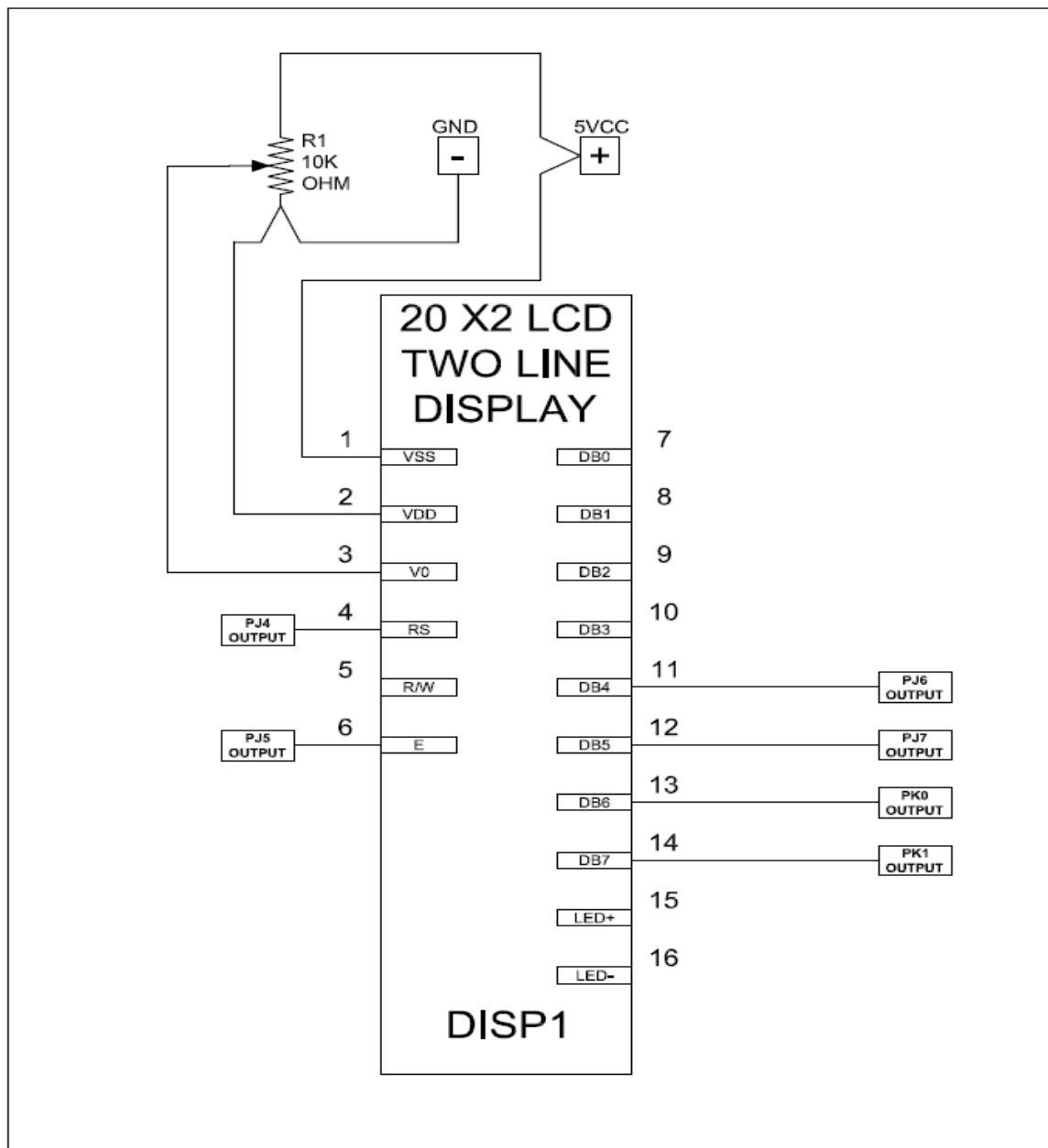
Figure 3.4-3: The electrical connections for the HMI # 1 user LCD twenty digit by two line display. This picture was drawn using AutoCAD educational software.
