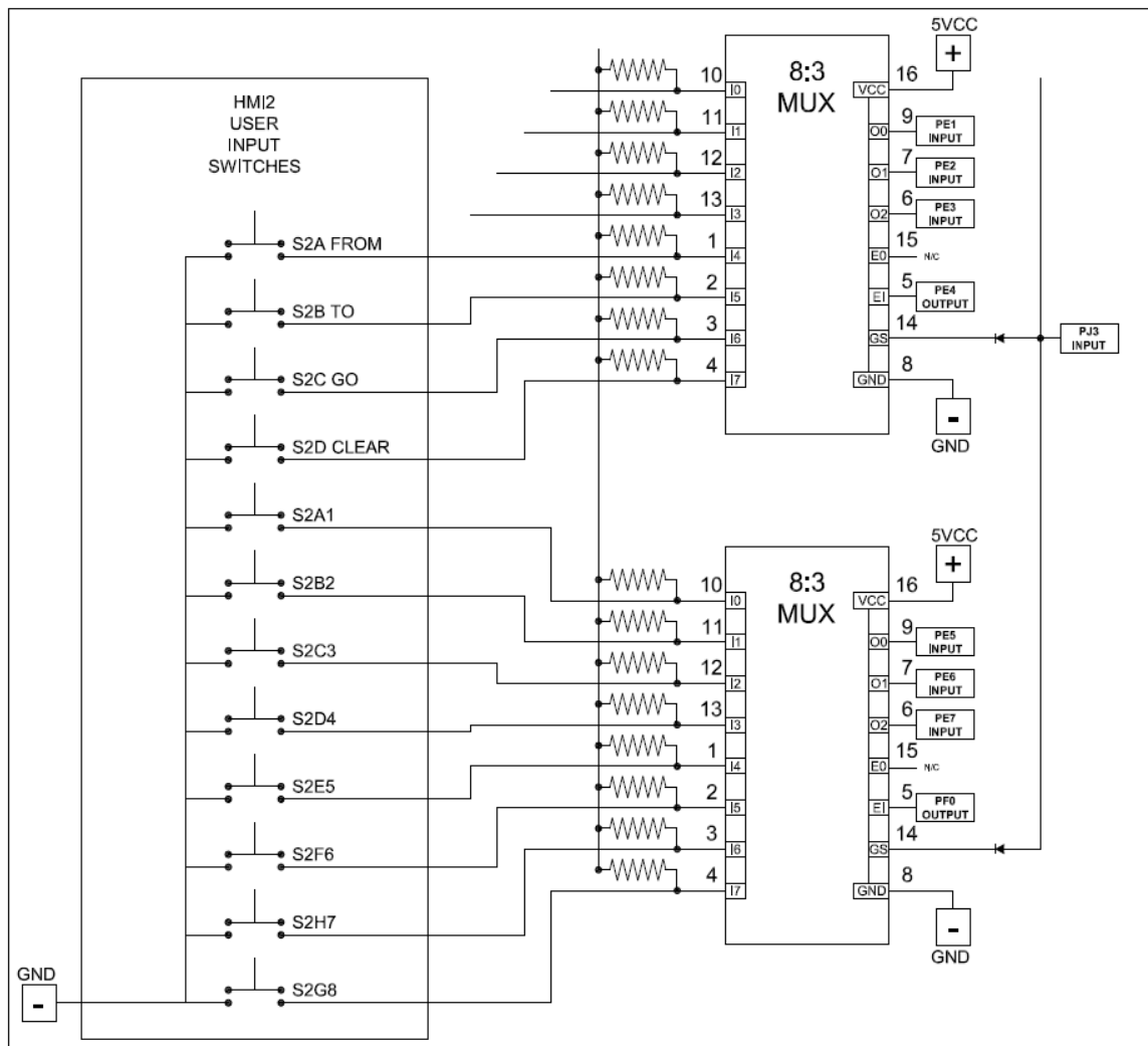
Figure 3.4-2: The design for the 5KΩ resistors and how they are electrically connected to the I/O panels. This picture was drawn using AutoCAD educational
