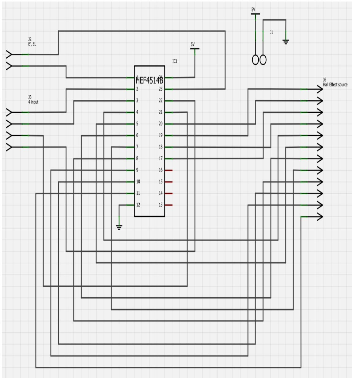
Figure 4.2.6-2: The schematic view for the independent boarding of the demultiplexer. This figure was created using Fritzing.
