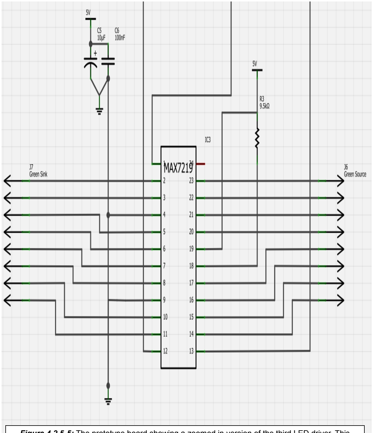
Figure 4.2.5-5: The prototype board showing a zoomed in version of the third LED driver. This figure was created using Fritzing.
