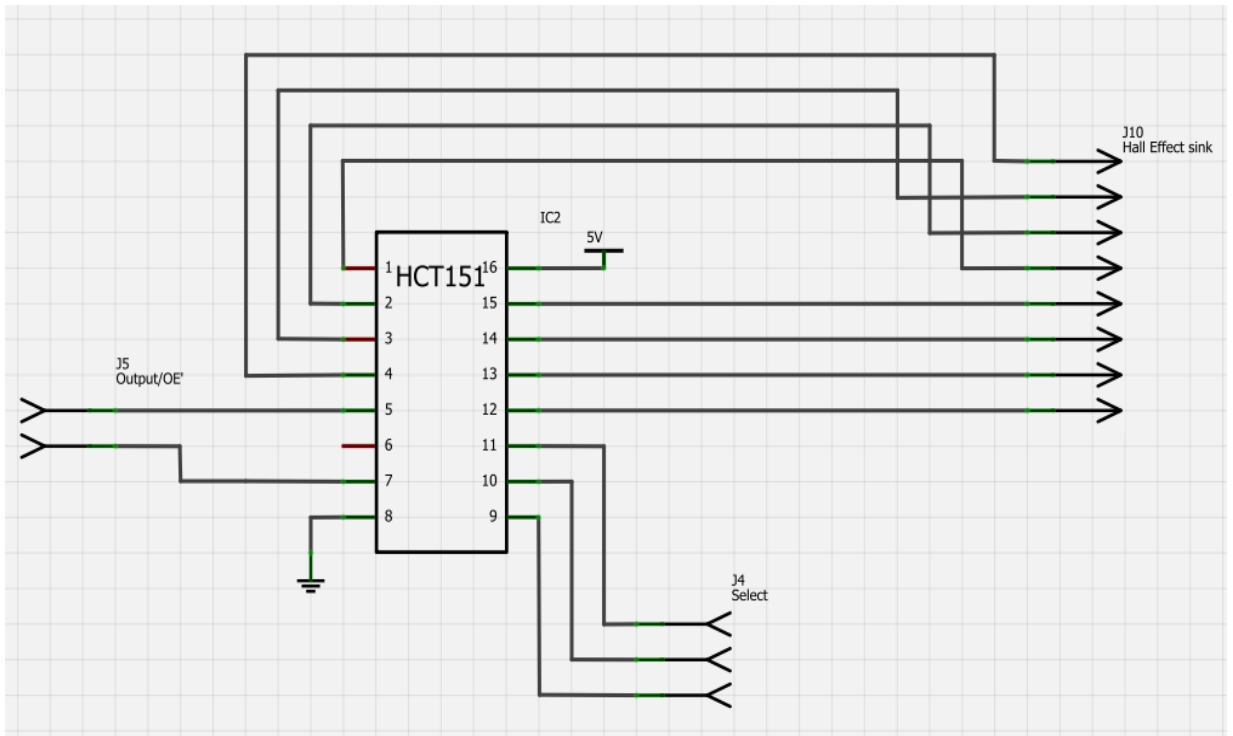
Figure 4.2.6-3: The schematic view for the independent boarding of the multiplexer. This figure was created using Fritzing.
