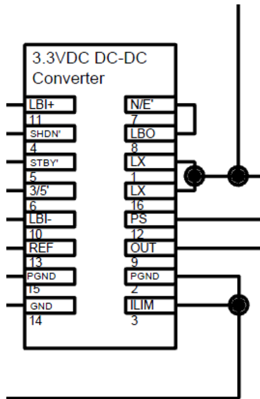
Figure 2.12-4: The 3.3 volt DC to DC converter; a MAX710 surface mounted chip
