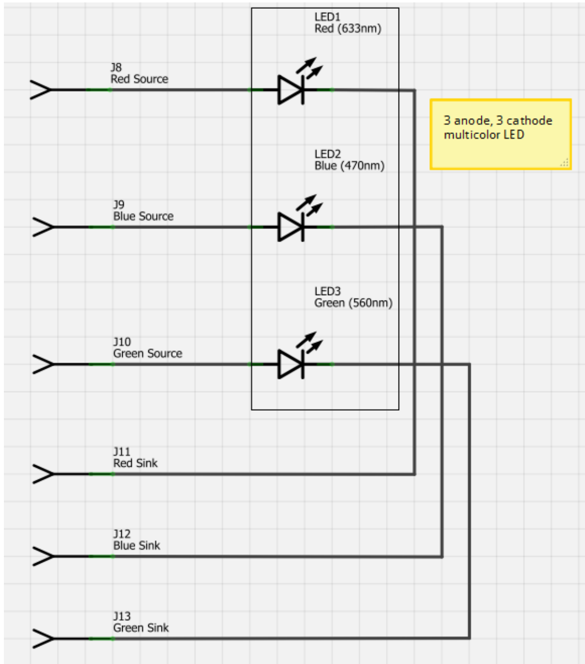
Figure 4.2.5-6: The schematic view of each LED on a separate individual board depicting each source and sink. This figure was created using Fritzing.
