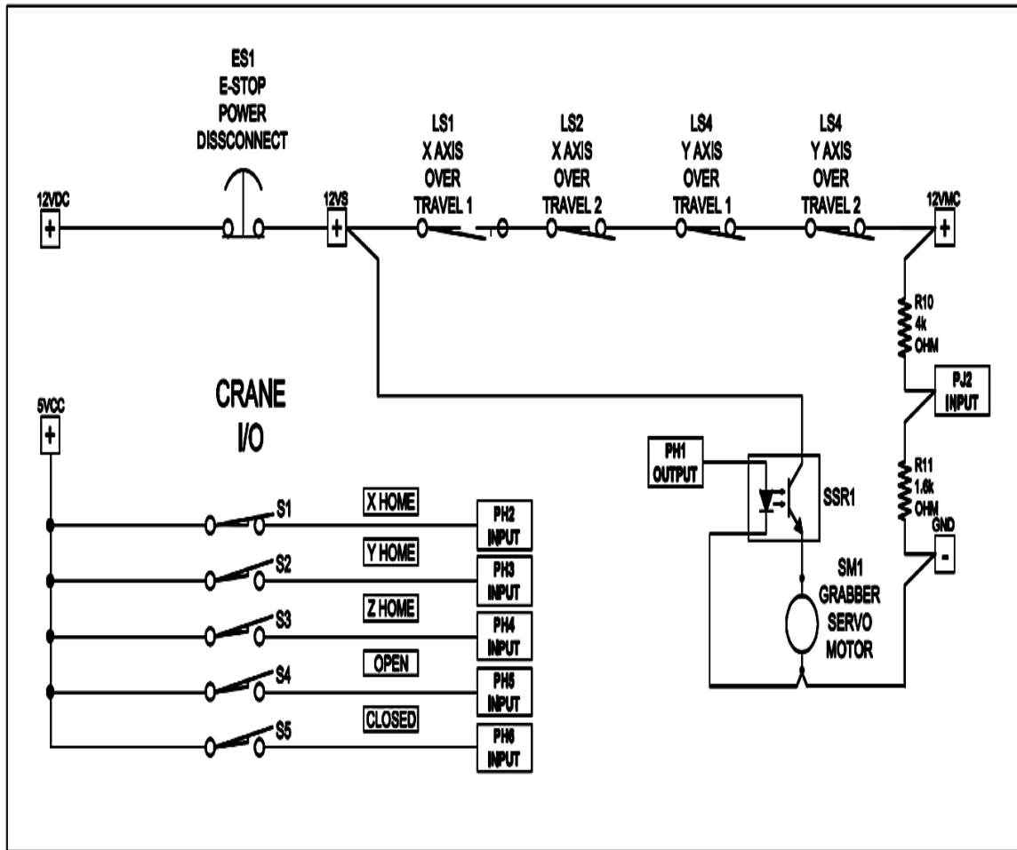
Figure 3.9.3-1: Control circuits for motion control. This picture was drawn using AutoCAD educational software.
