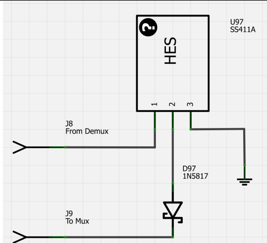
Figure 4.2.6-4: The schematic view for the sensor board. This figure was created using Fritzing.
