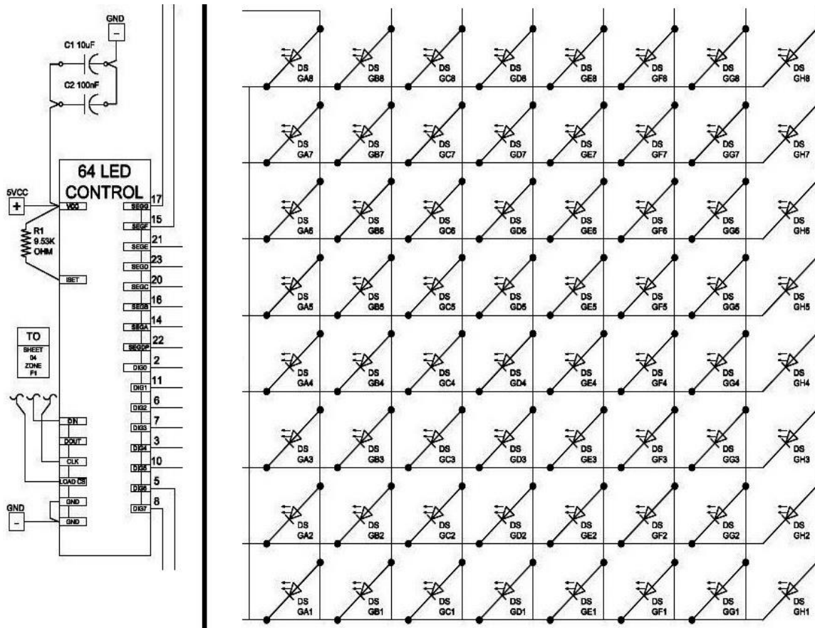
Figure 3.6-7: The essential components for the green LED schematic zoomed in for easy reading. This figure was created using AutoCAD educational software.
