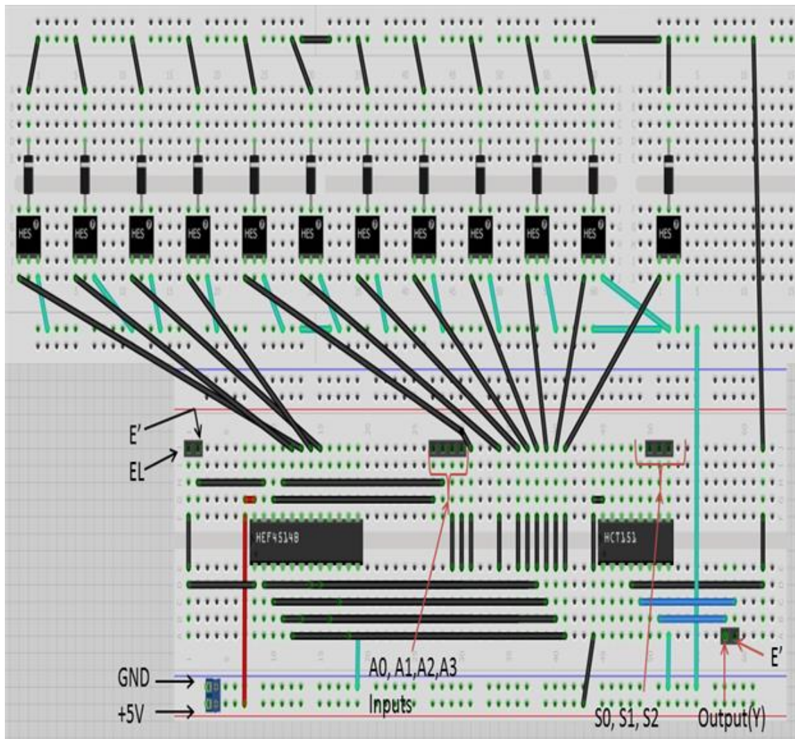
Figure 4.2.6-1: The schematic view of the Hall Effect Matrix grid's set up. This figure was created using Fritzing.
