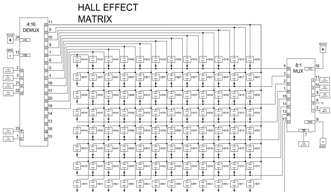
Figure 3.6-2: The full view of the final Hall Effect sensor grid. This figure was created using AutoCAD educational software.
