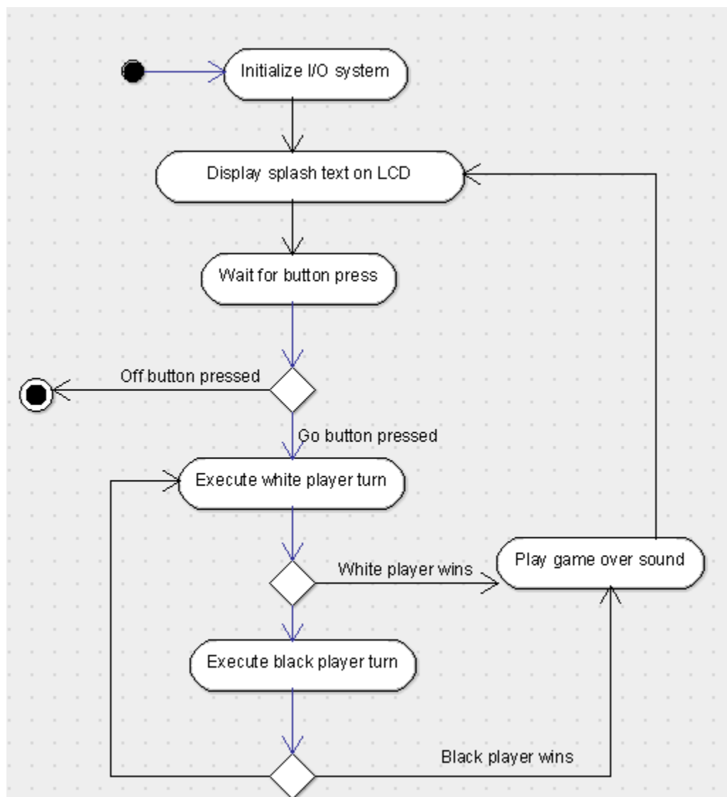
Figure 3.3.3.2-1: Main module activity diagram
