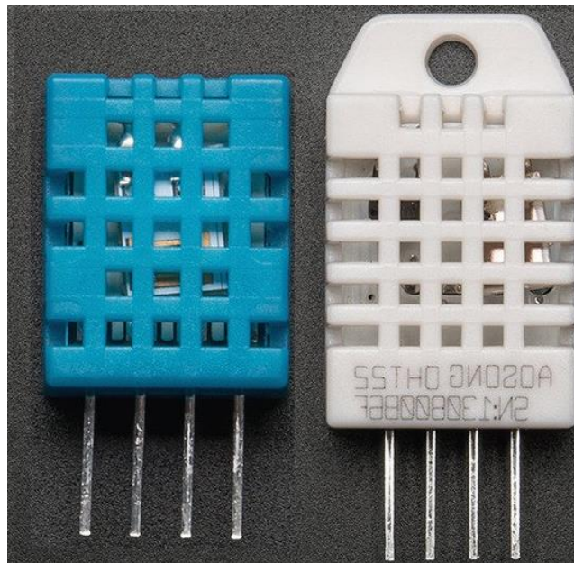
Figure 3.8.1. Left: DHT11 Right: DHT22
