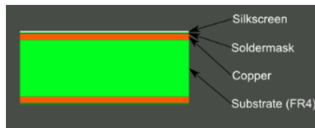
Figure 3.4.1. Cross-section of a Printed Circuit Board
