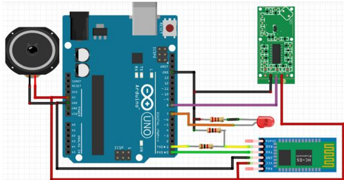
Figure 7.3.1.1 Security Mode Breadboard built in Fritzing software
