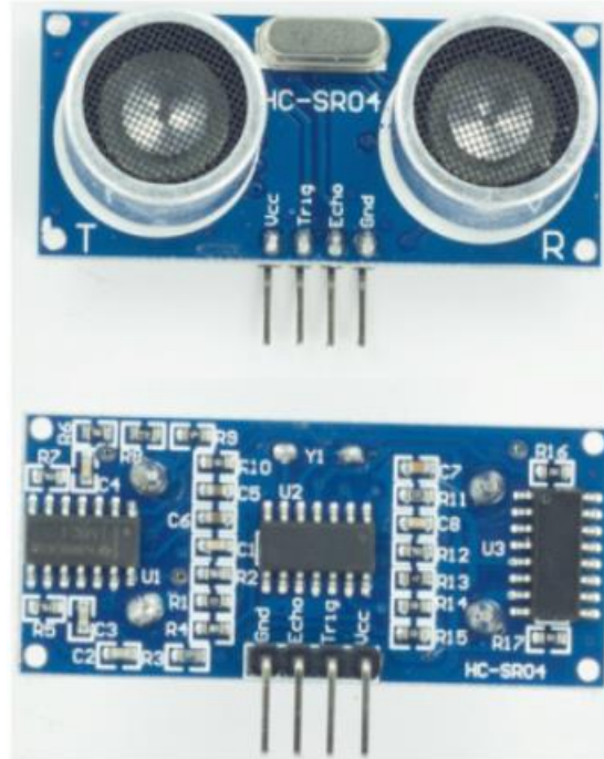
Figure 3.7.2. Ultrasonic Sensor Module
