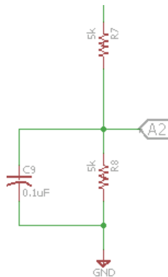
Figure 5.2.4 Voltage Sensor for Reading Battery Voltage Schematic
