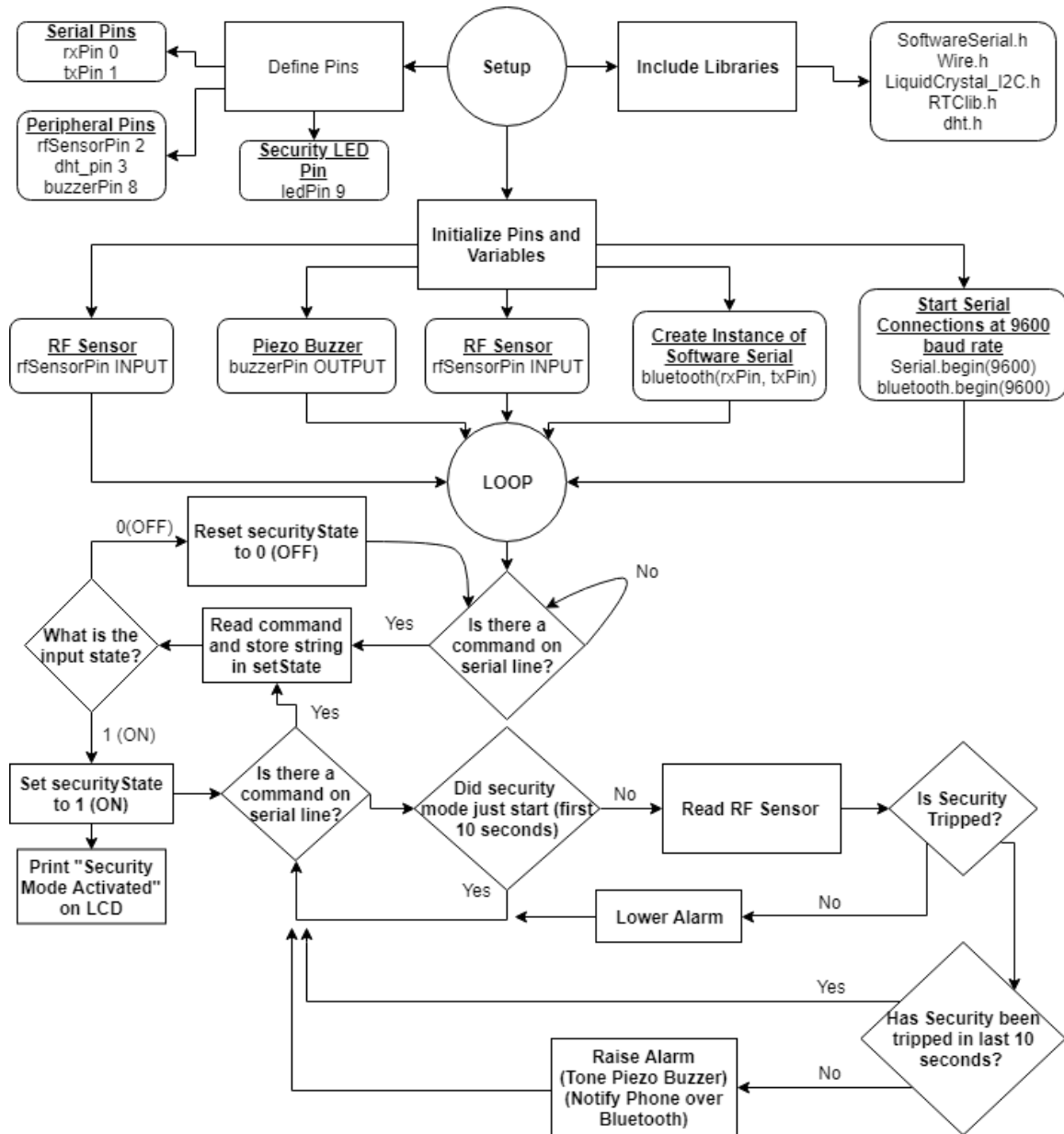
Figure 6.2.1. Flowchart for Security Mode Design
