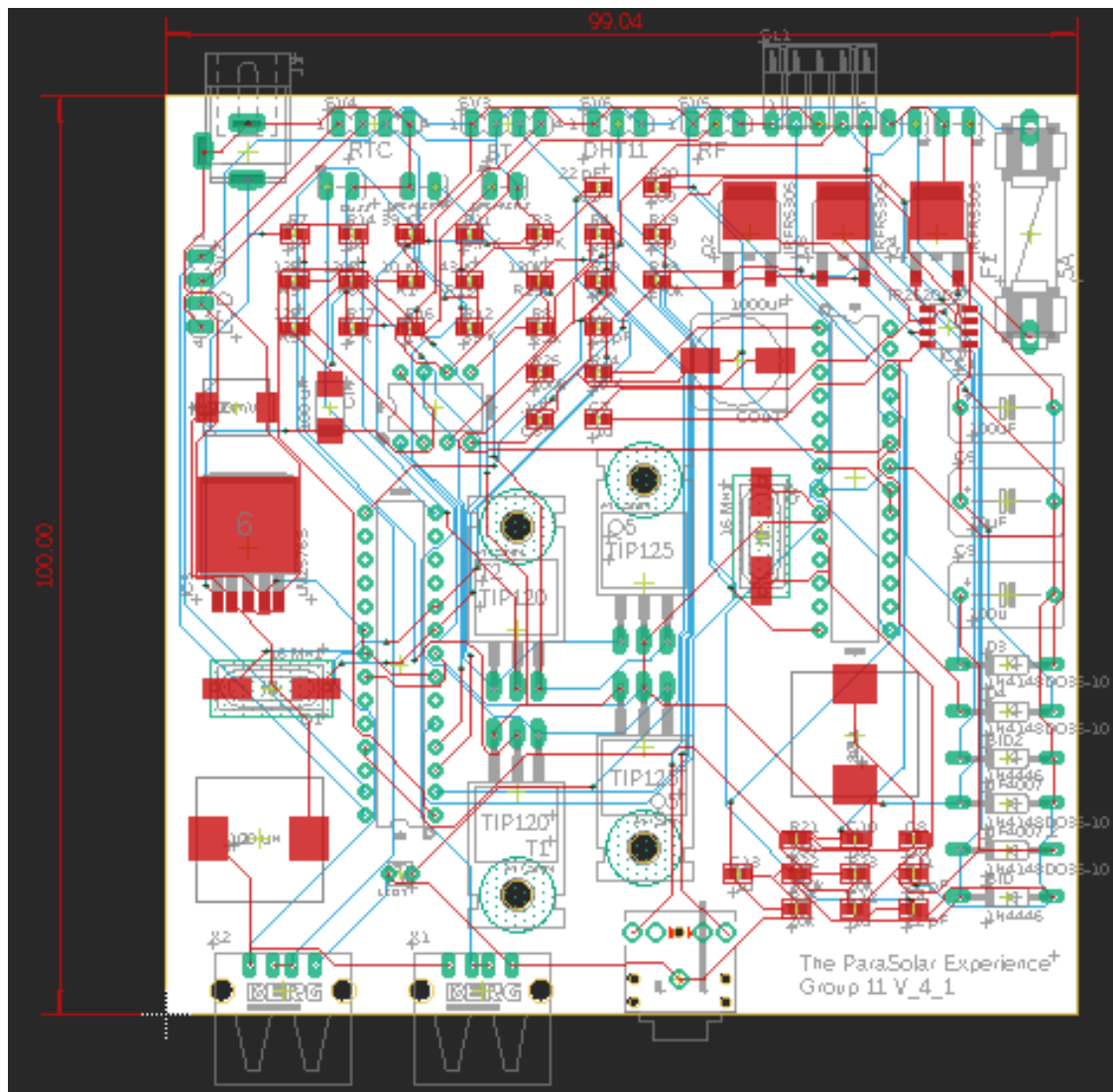
Figure 3. Complete PCB Footprint
