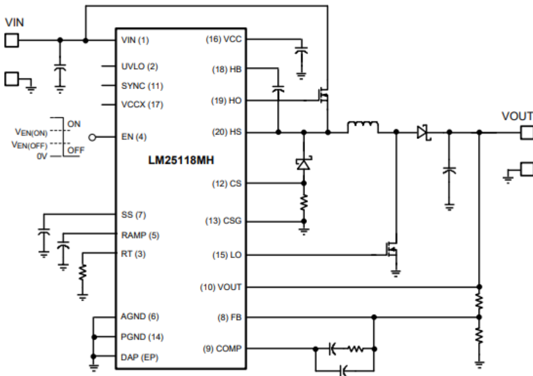
Figure 3.5.8. Source to 12V circuit design diagram
