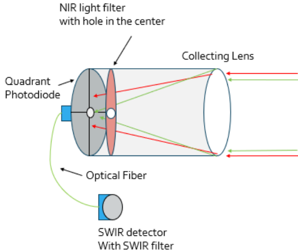
Fig 4: Diagram of the optical layout for the receiver side
