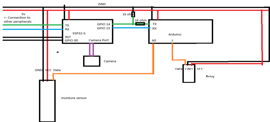
Figure 9.1: Full breadboard integration
