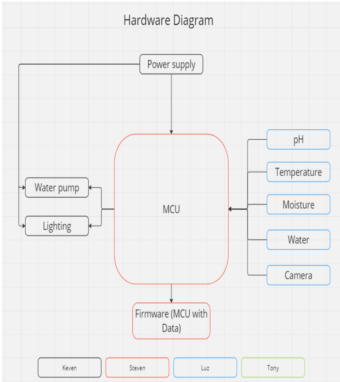
Figure 2.1: Hardware Diagram
