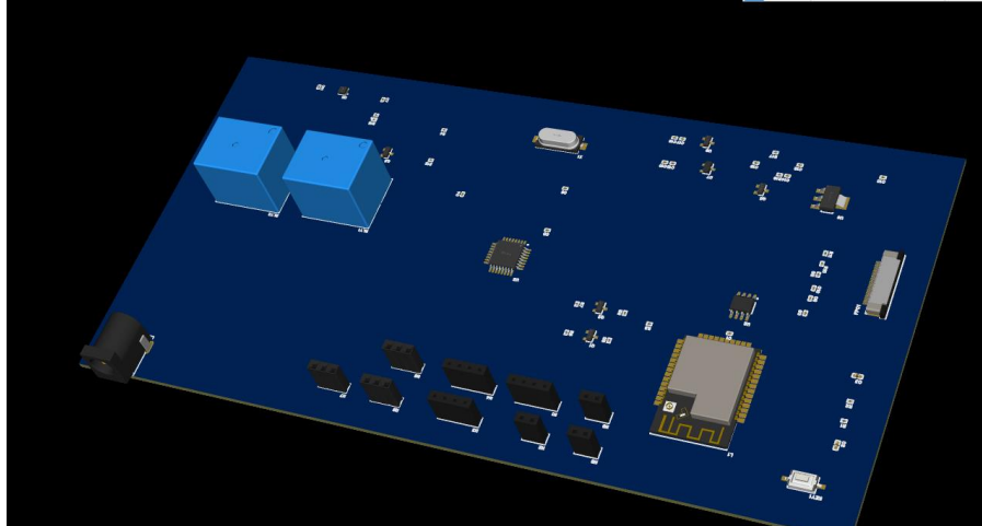
Figure 8.1: The 3d render of the PCB
