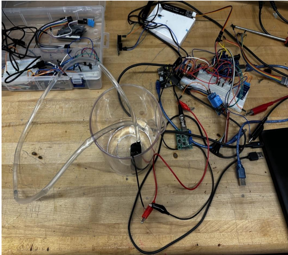
Figure 9.1: Full breadboard integration
