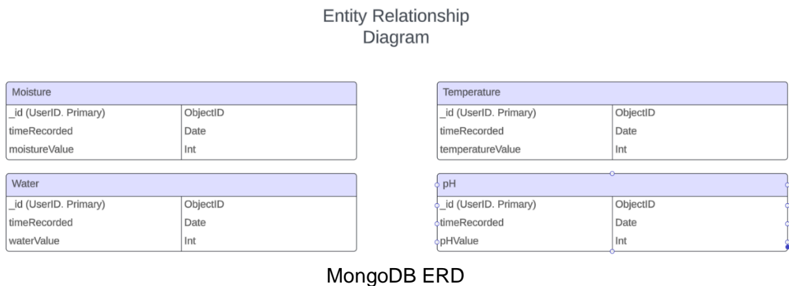
Figure 7.3: MongoDB ERD
