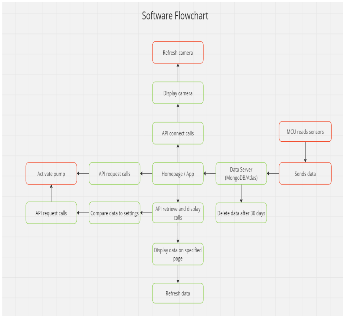
Figure 7.2: Software/App Flowchart
