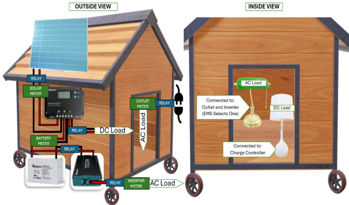
Figure 28: Smart Home Model Structural Illustration
