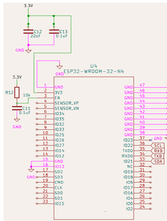
Figure 24: ESP32 Schematic for Solar Panel Metering PCB
