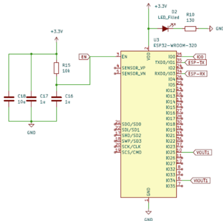
Figure 12: Schematic of Microcontroller Unit with Measurement Connections
