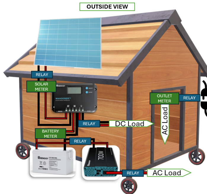
Figure 47: Prototype Including Relays and Metering Devices
