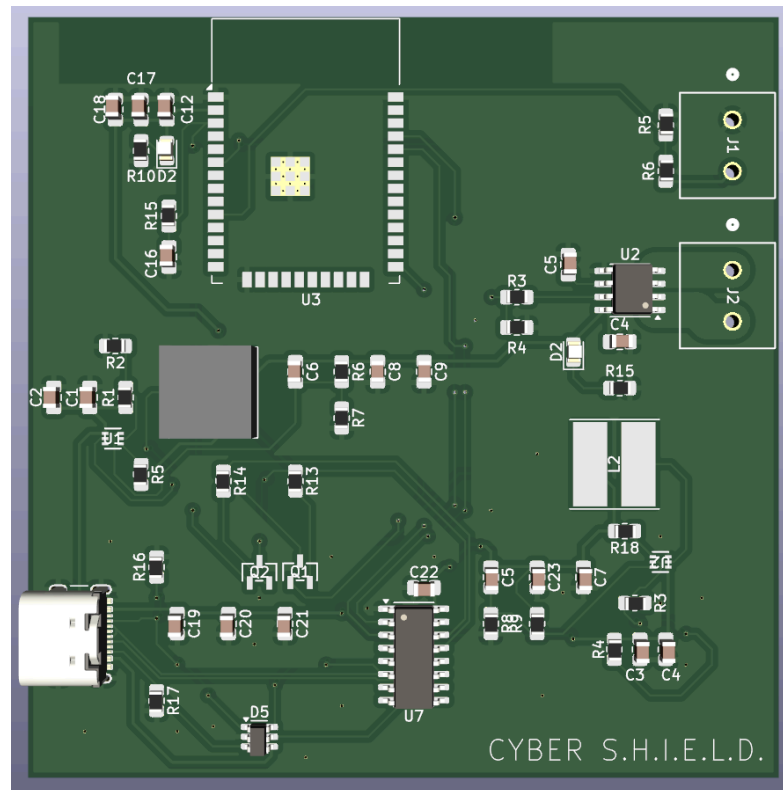
Figure 44: 3D Model of Battery Metering PCB
