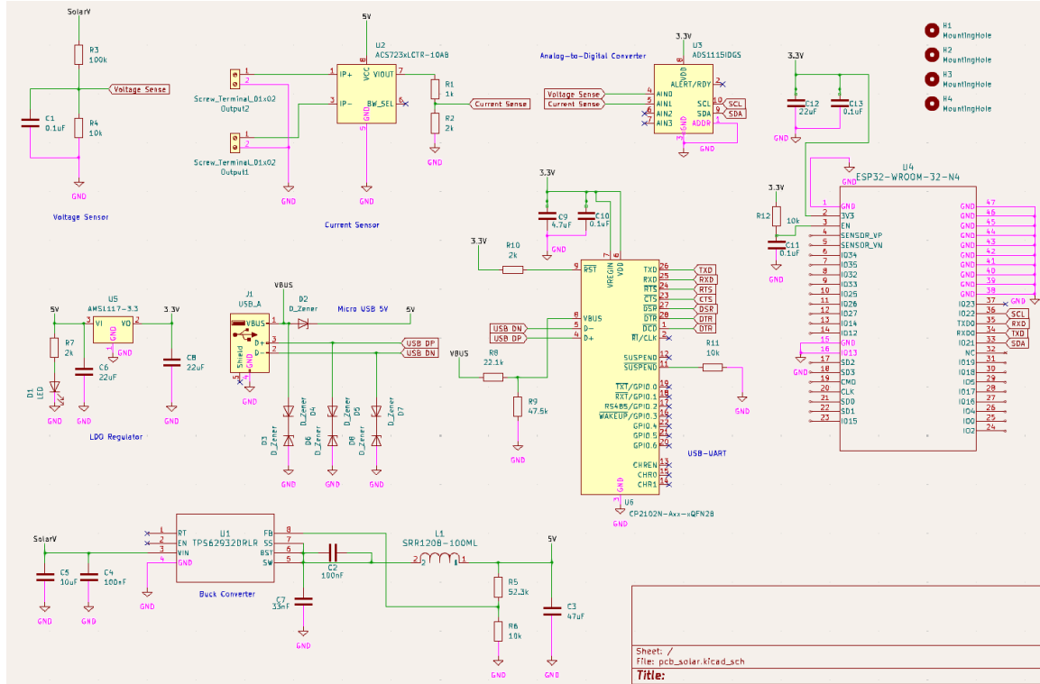
Figure 25: Completed Schematic for Solar Panel Metering PCB
