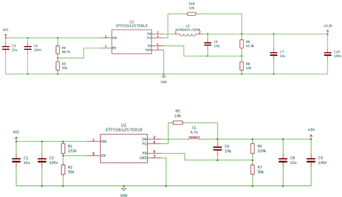
Figure 15: Power Supply Connections
