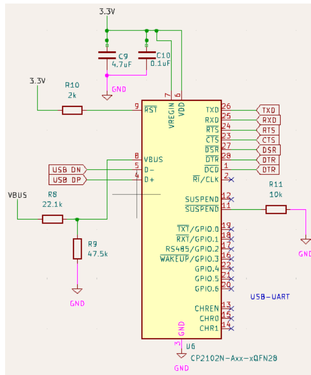
Figure 22: USB-UART Schematic for Solar Metering PCB
