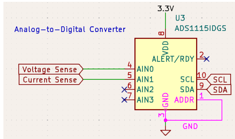
Figure 23: ADC Schematic for the Solar Panel Metering PCB
