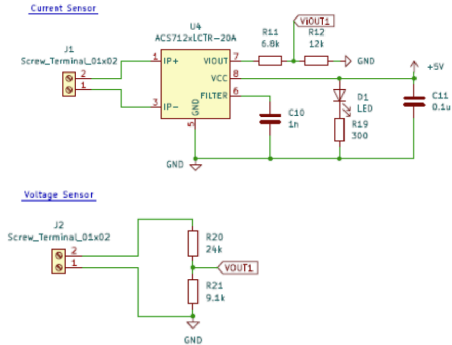
Figure 13: Current and Voltage Sensor Circuits
