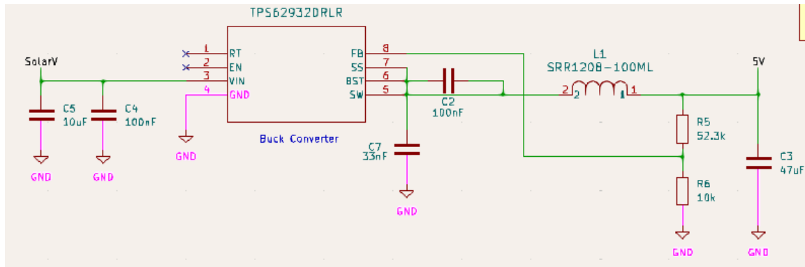
Figure 17: Buck Converter for Solar Panel Metering PCB
