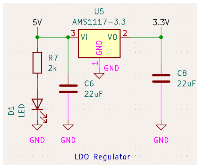
Figure 20: LDO Regulator for Solar Panel Metering PCB
