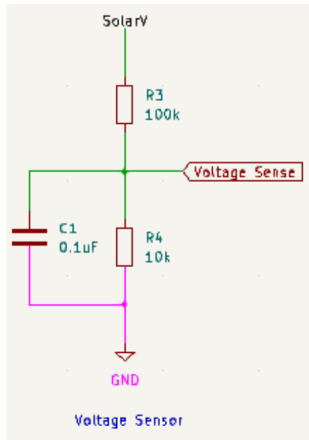
Figure 19: Voltage Sensor for Solar Panel Metering PCB
