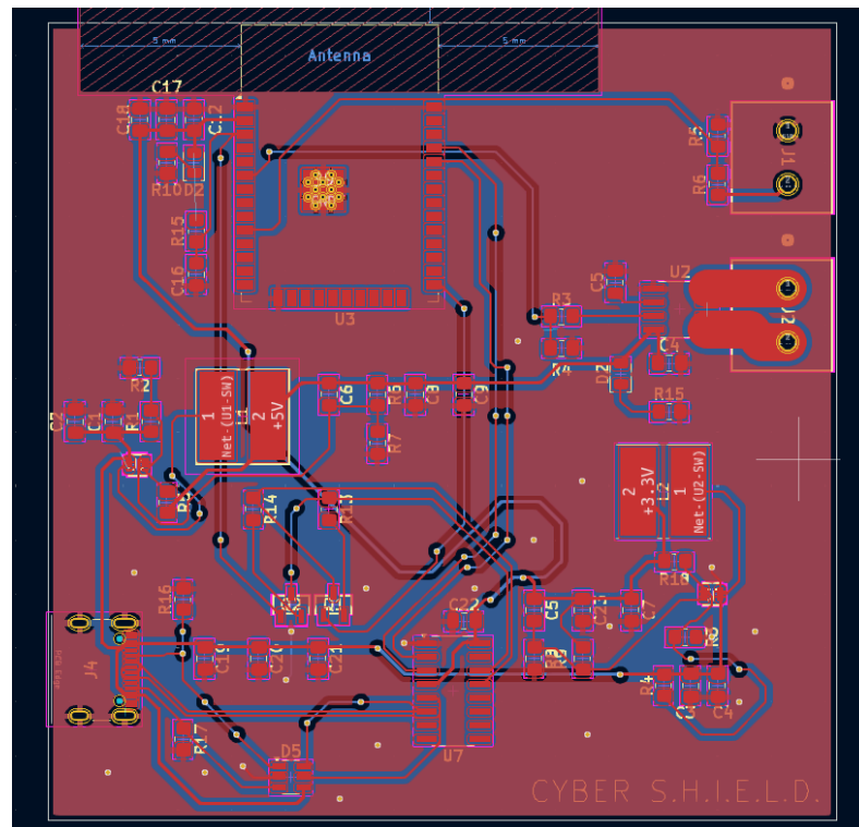
Figure 43: Battery Metering PCB Layout
