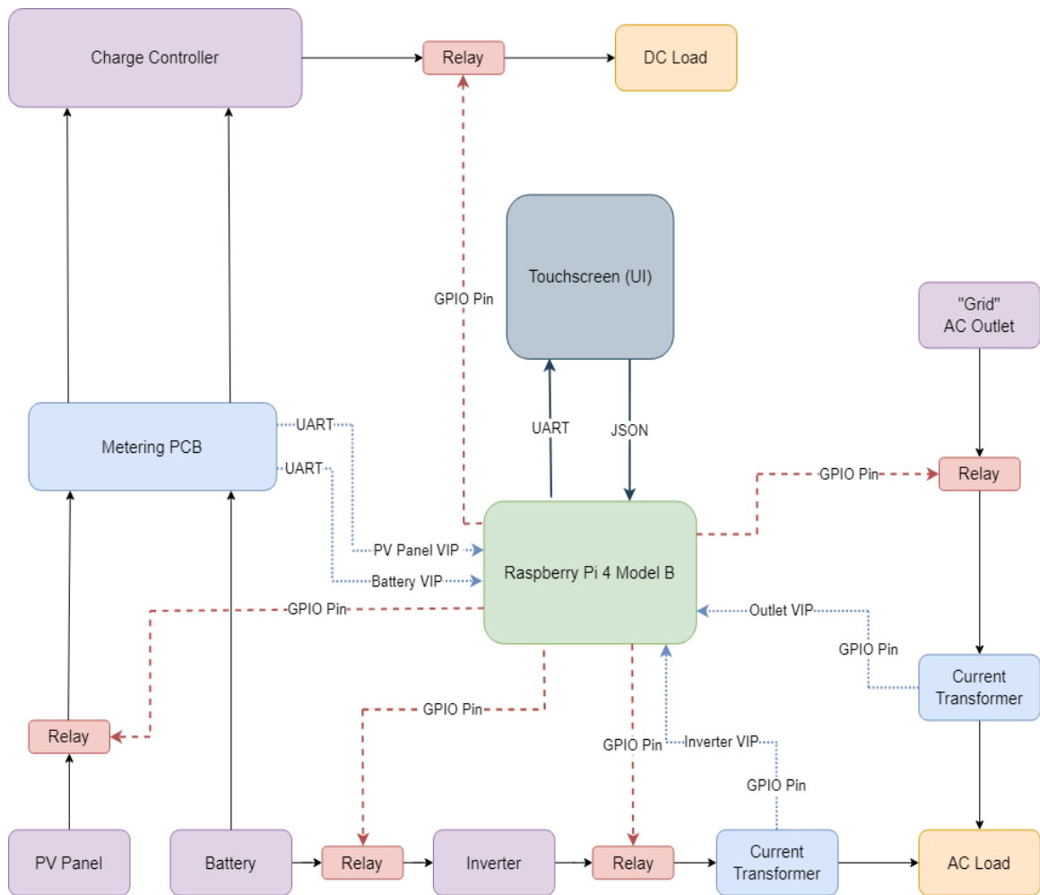
Figure 26: System Architecture
