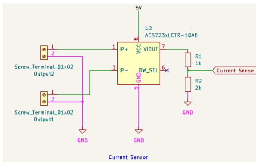
Figure 18: Current Sensor for Solar Panel Metering PCB
