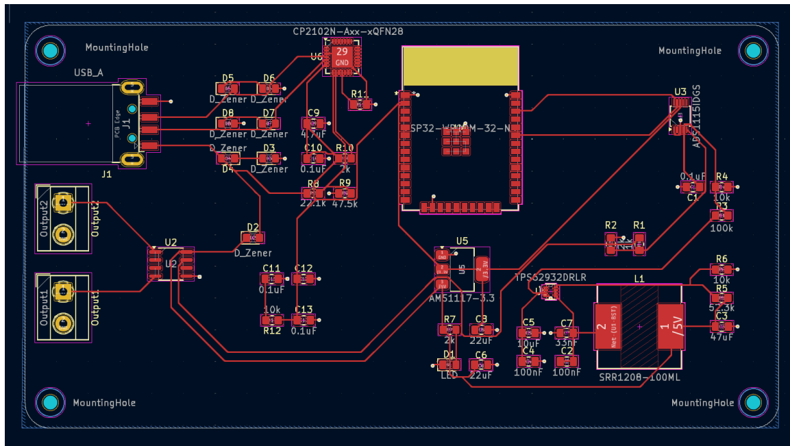
Figure 41: Solar Panel Metering PCB Layout
