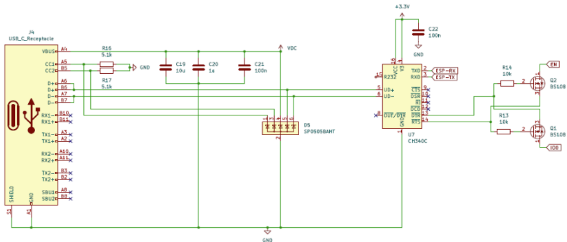
Figure 14: USB Connections
