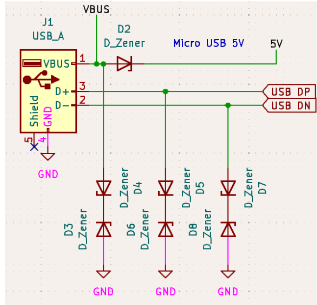
Figure 21: Micro USB Schematic for Solar Metering PCB
