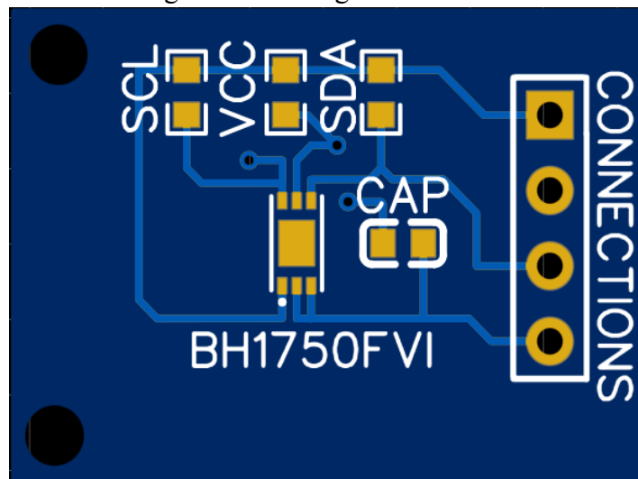
Figure 8.2.1.2 2D Light Sensor Overview
