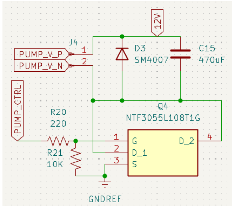
Figure 6.1.3.1 Pump Driver Schematic
