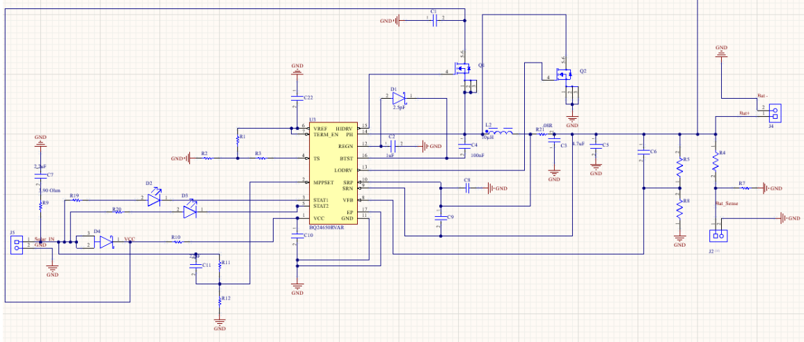
Figure 6.1.6.3 Charge Controller Schematic.
