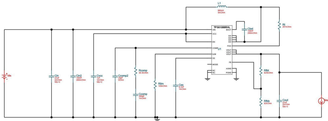
Figure 6.1.5.2.1 Boost Converter
