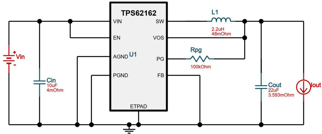
Figure 6.1.5.2.2 Buck Converter
