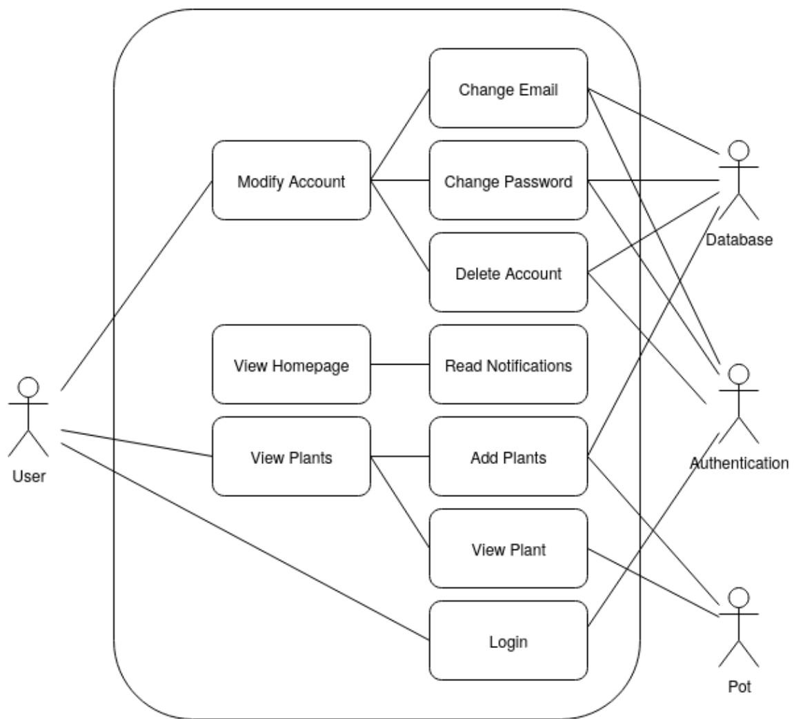
Figure 7.7.1.1 Use Case Diagram for Web Server Client
