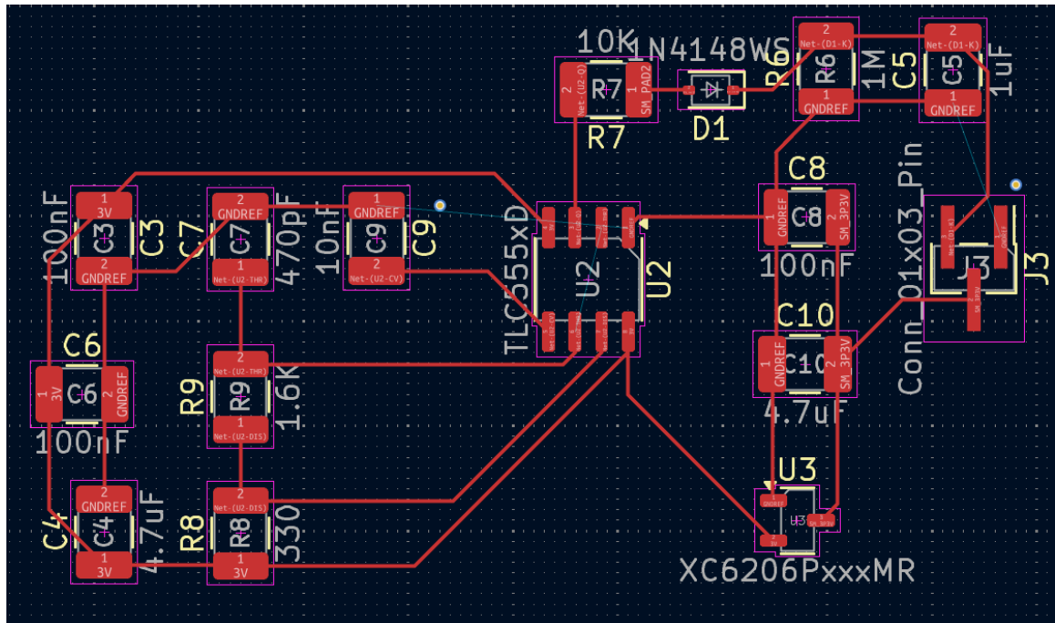
Figure 8.2.3.1 Soil Moisture Sensor PCB Design.
