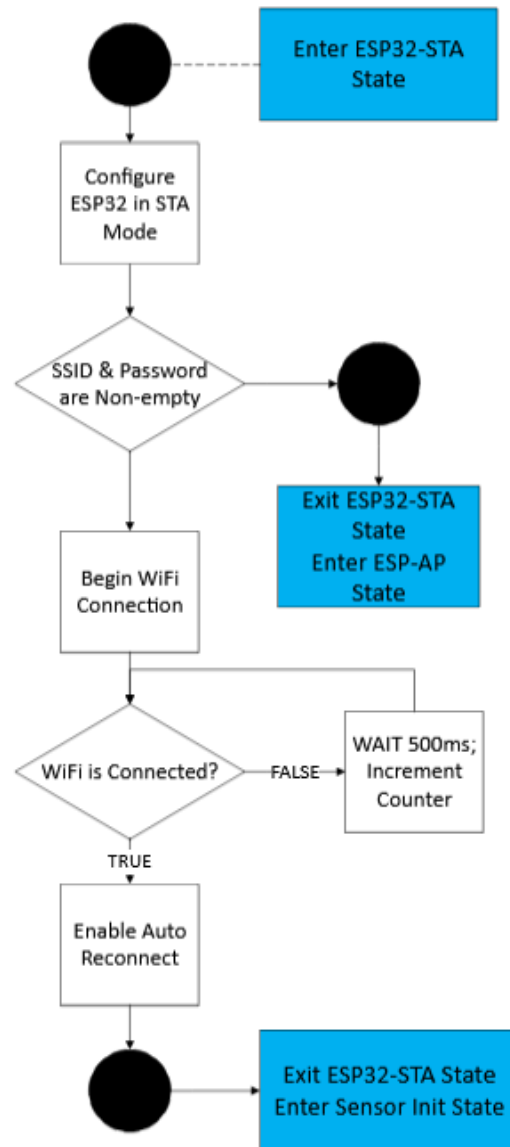
Figure 7.2.3 Activity Diagram for ESP32-STA State.
