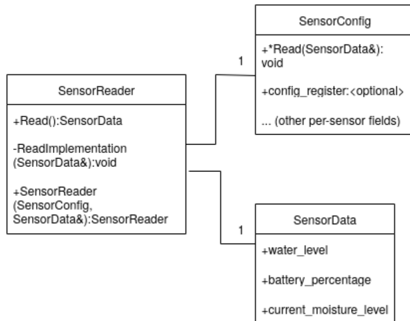
Figure 7.4.2 SensorReader Class Diagram
