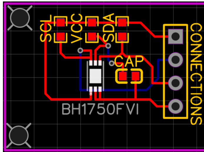
Figure 8.2.1.1 Light Sensor PCB
