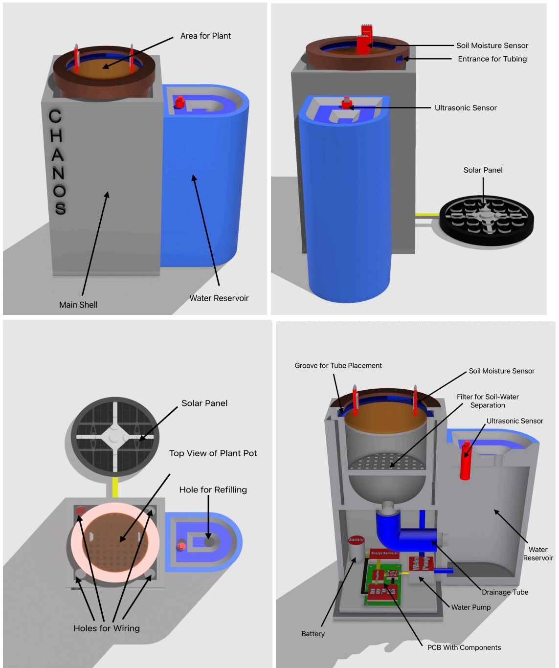
Figure 2.6, top left, front view (a), top right, side view (b), bottom left, top view (c), and bottom right, internal view (d), of C.H.A.N.O.S.
