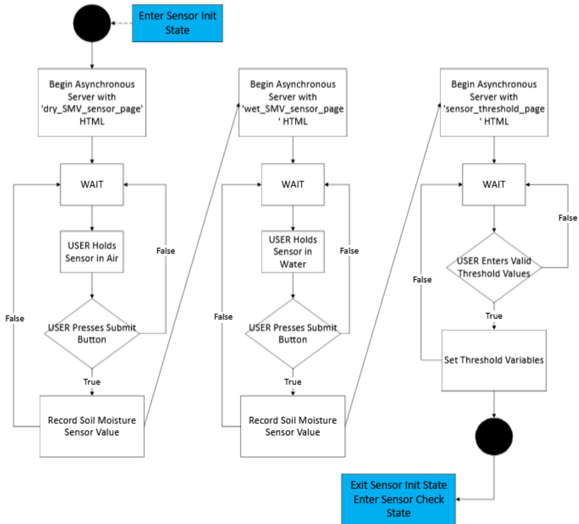
Figure 7.2.4 Activity Diagram for Sensor Init State.
