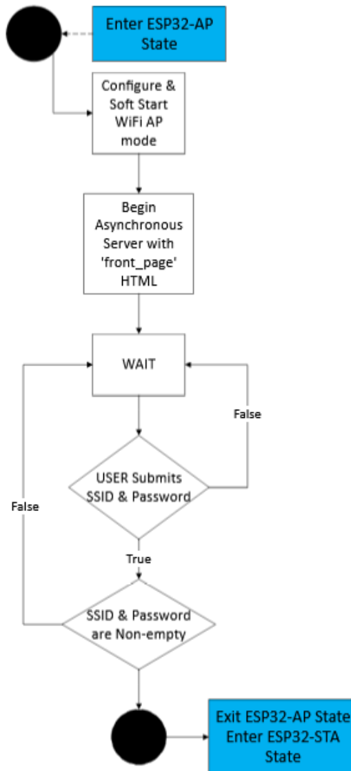
Figure 7.2.2 Activity Diagram for ESP32-AP State.
