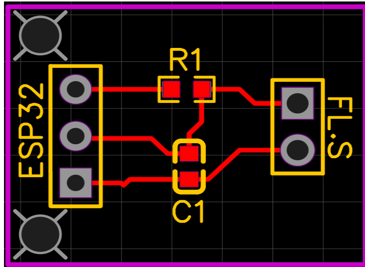
Figure 8.2.2.1 Water Level Sensor PCB
