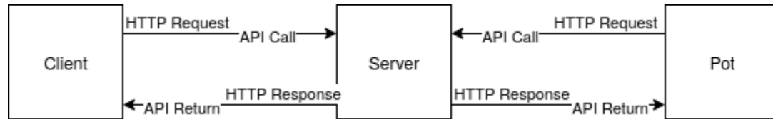
Figure 7.7.2.1 Server API Message Flow
