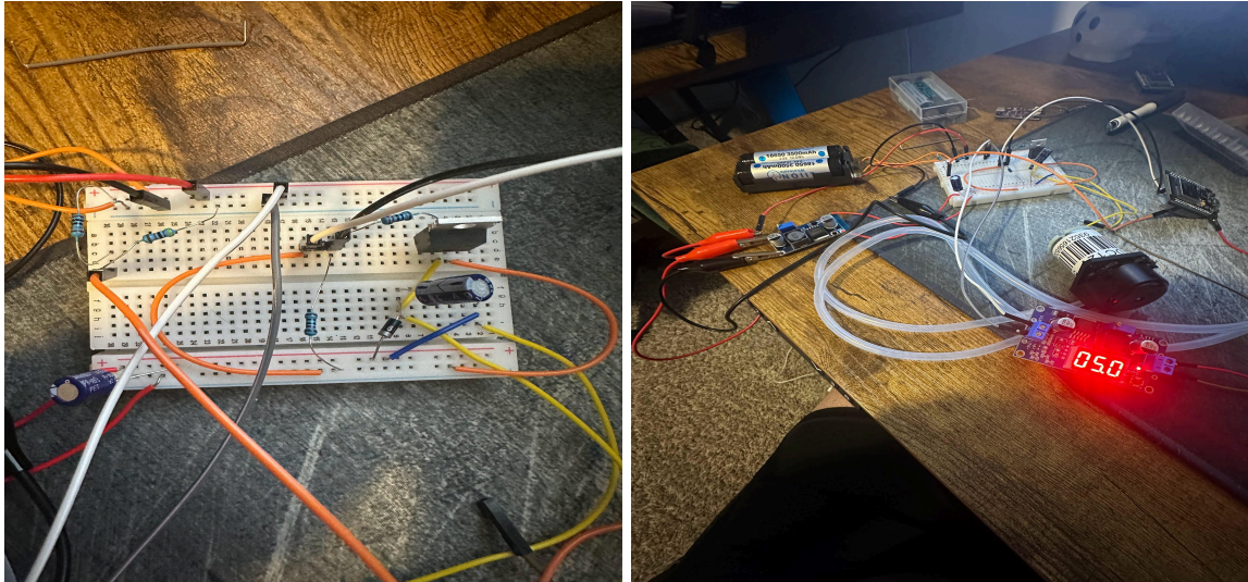
Figure 9.1.1 Breadboard Testing
