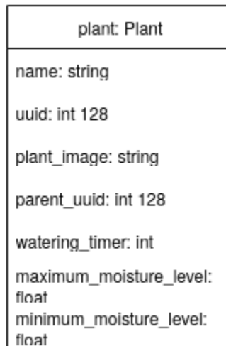
Figure 7.3.1.2 Plant Data Structure Diagram.
