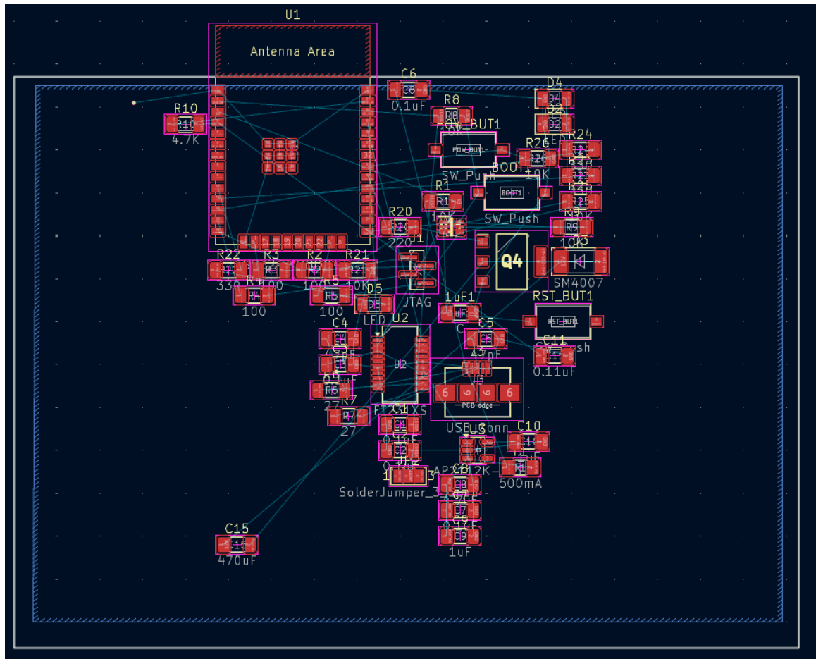
Figure 8.2.4.1 MCU and UART-USB PCB Design.
