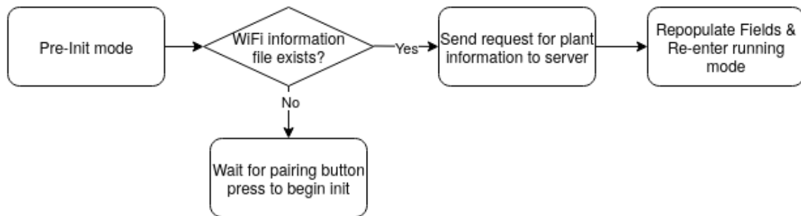
Figure 7.1.2.1 Power-Loss Restoration Flowchart.
