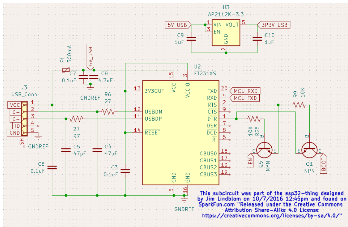
Figure 6.1.7.1 USB-UART Conversion Schematic.
