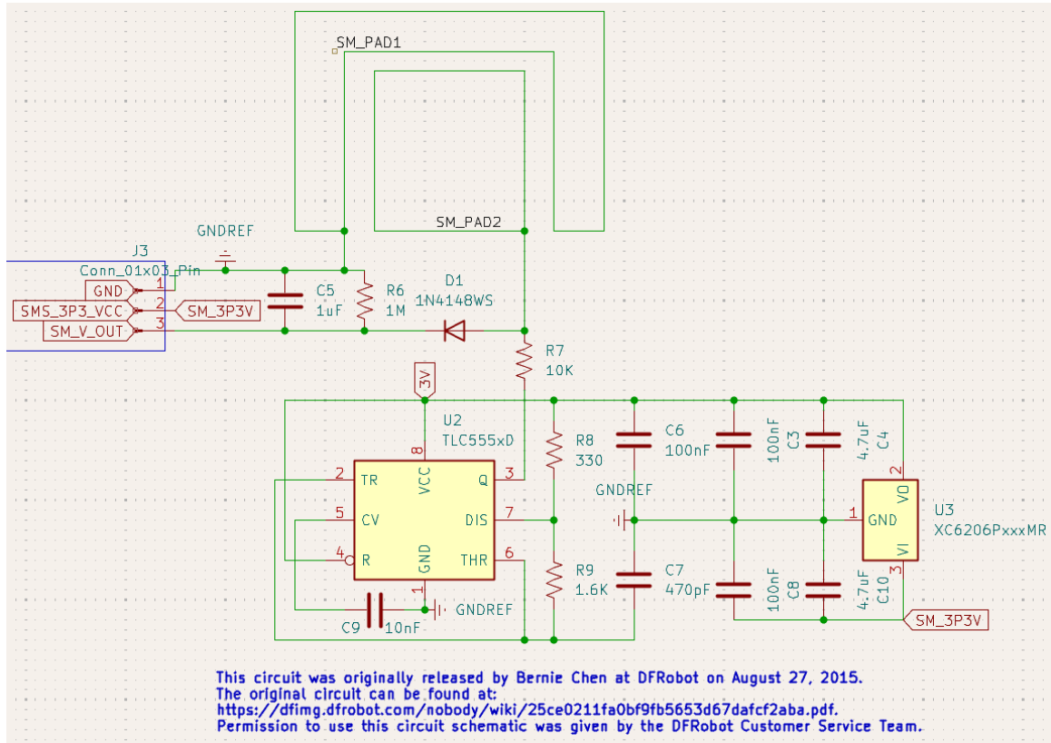
Figure 6.1.4.2.1. Soil Moisture Sensor Schematic.
