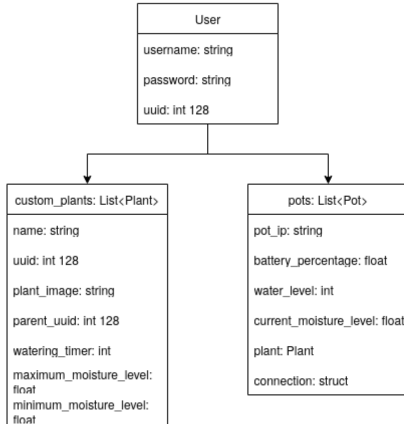
Figure 7.3.3.2 User Data Structure Diagram.
