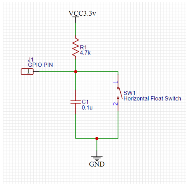
Figure 6.1.4.3.1 Water Level Sensor Schematic
