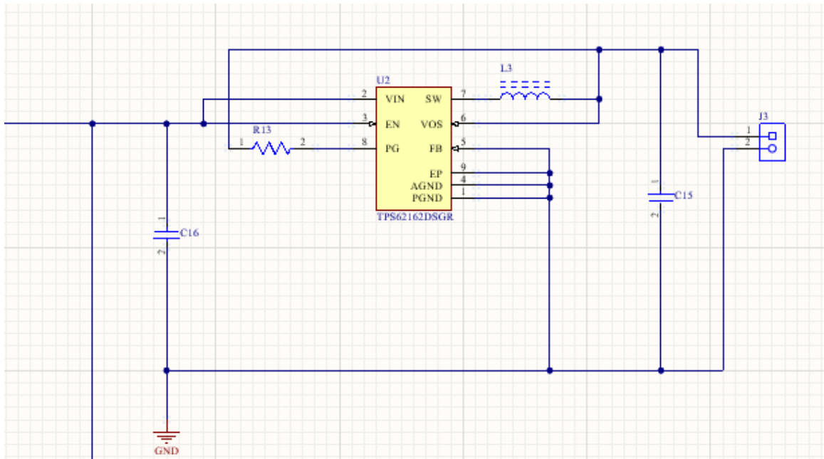
Figure 6.1.6.2 3.3V Buck Converter Schematic.
