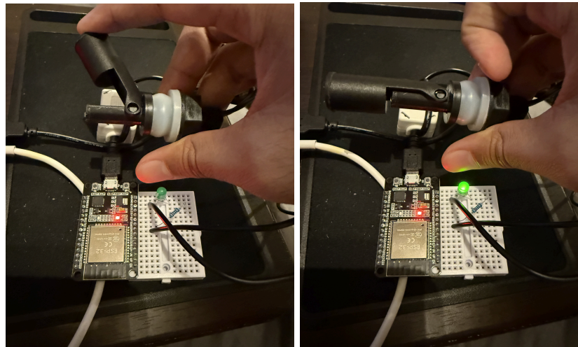
Figure 9.1.1.3.1 Horizontal Float Sensor Test
