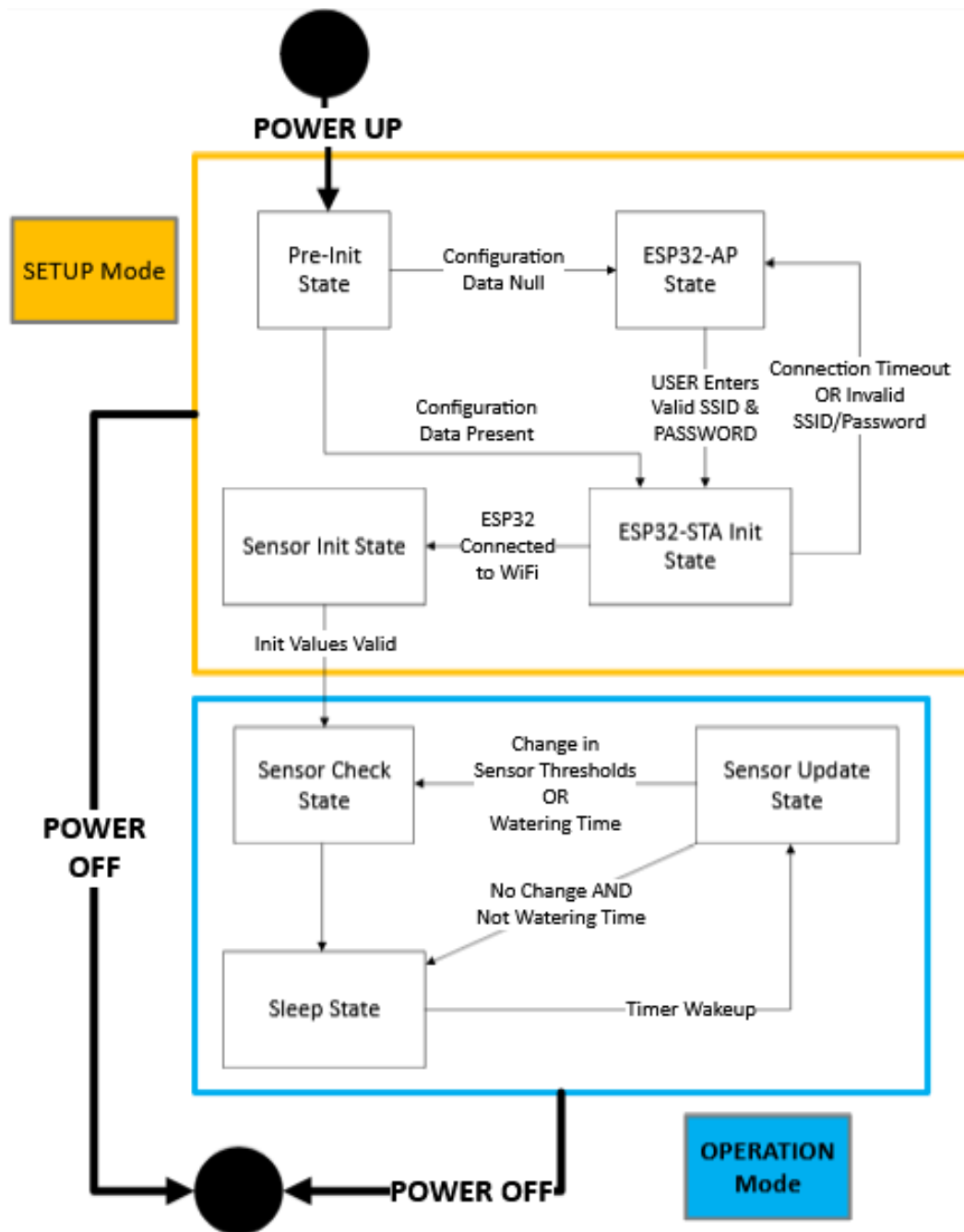
Figure 7.2.1 Overall Software State Diagram.
