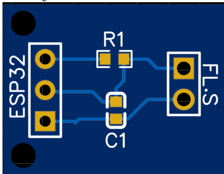
Figure 8.2.2.2 2D Horizontal Water Sensor
