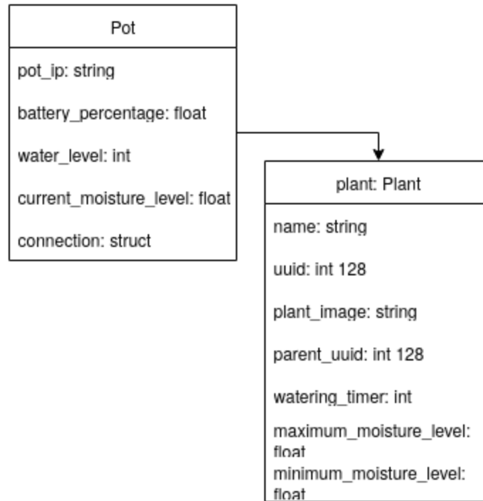
Figure 7.3.2.1 Pot Data Structure Diagram.
