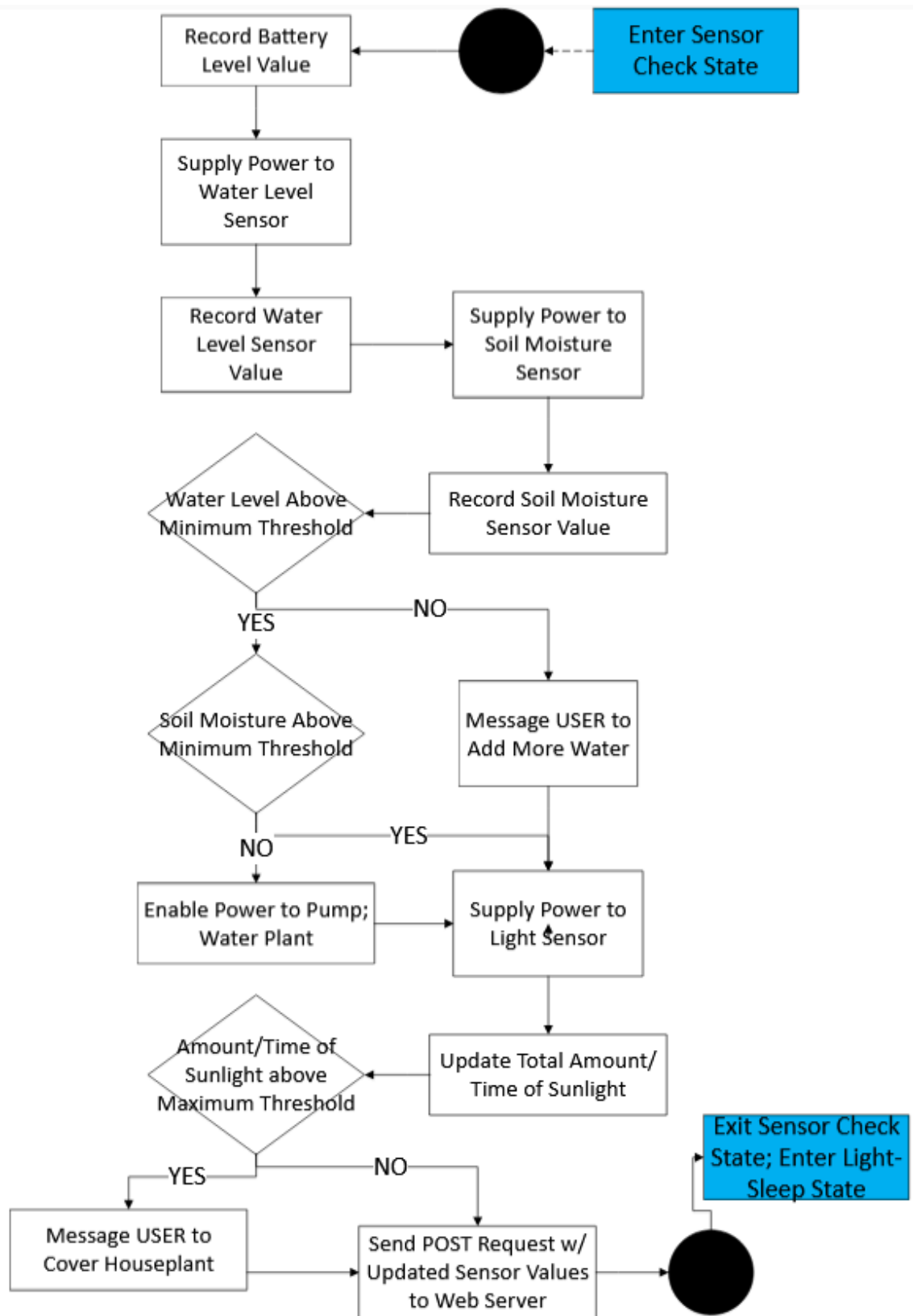
Figure 7.2.5 Activity Diagram for Sensor Check State.
