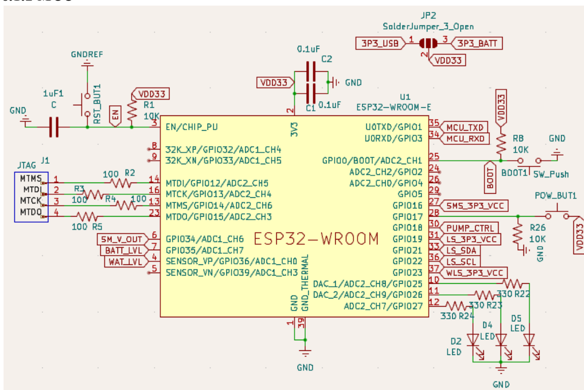
Figure 6.1.2.1 Microcontroller Schematic.
