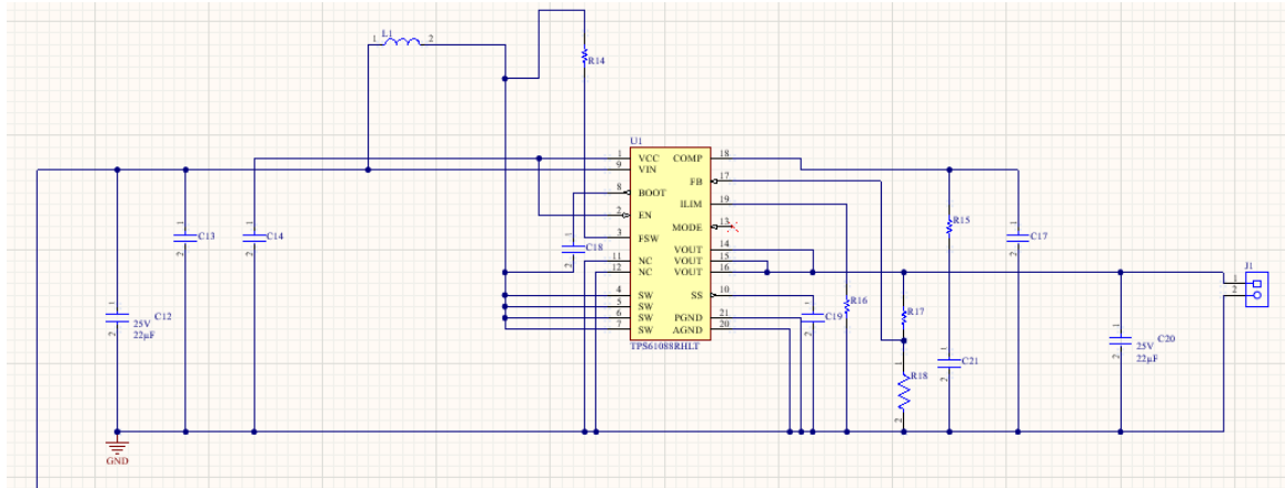
Figure 6.1.6.1 12V Boost Converter Schematic.
