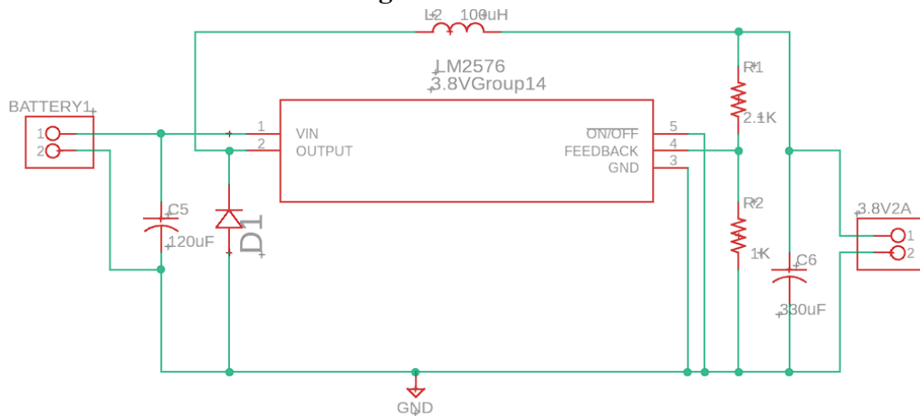
Figure 6.6 — SIM7600 and LiDAR Regulator (3.8V and 2A)
