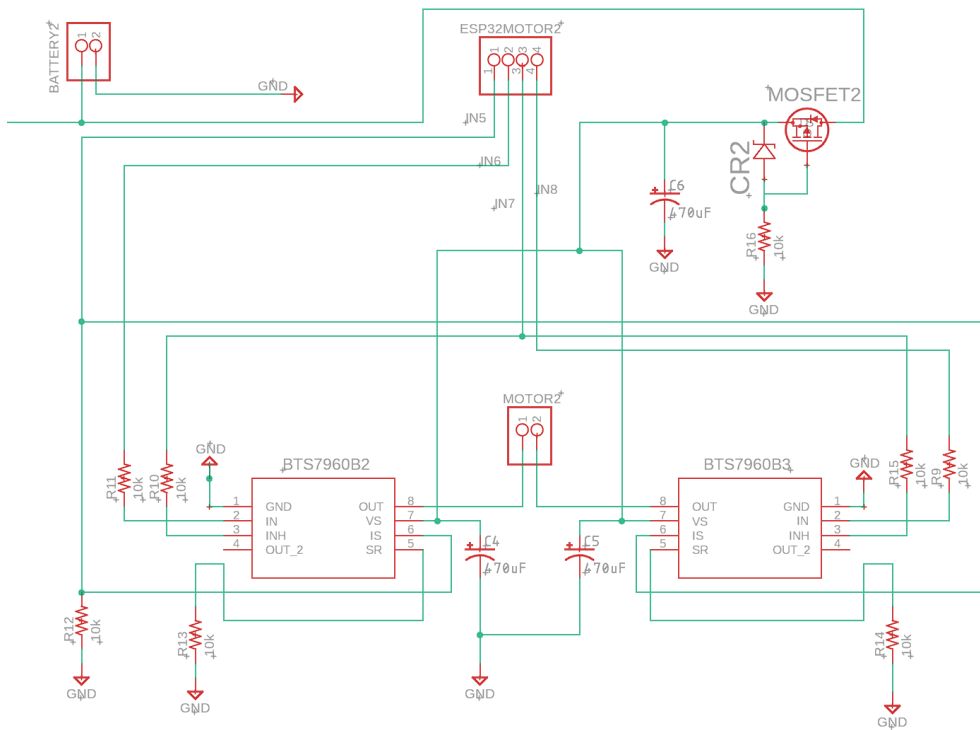
Figure 6.4 — Motor Controller (Right)
