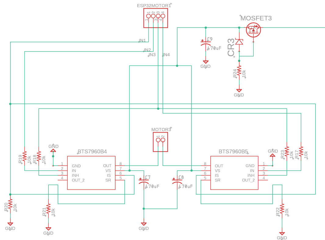
Figure 6.3 — Motor Controller (Left)
