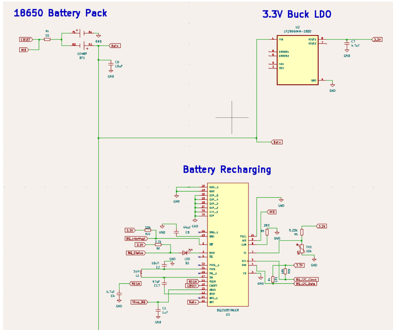
Schematic (1) for the User Output Device
