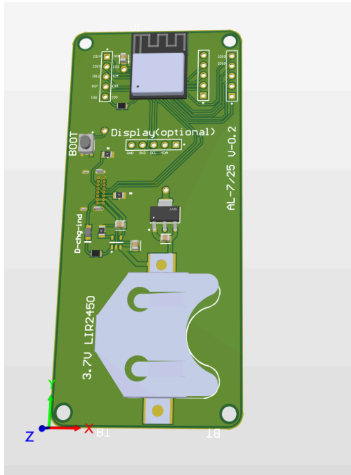
3D model of the User input Device
