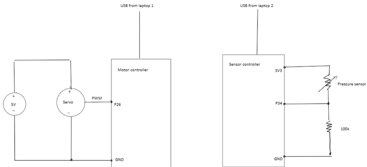
Wiring diagram for third trial
