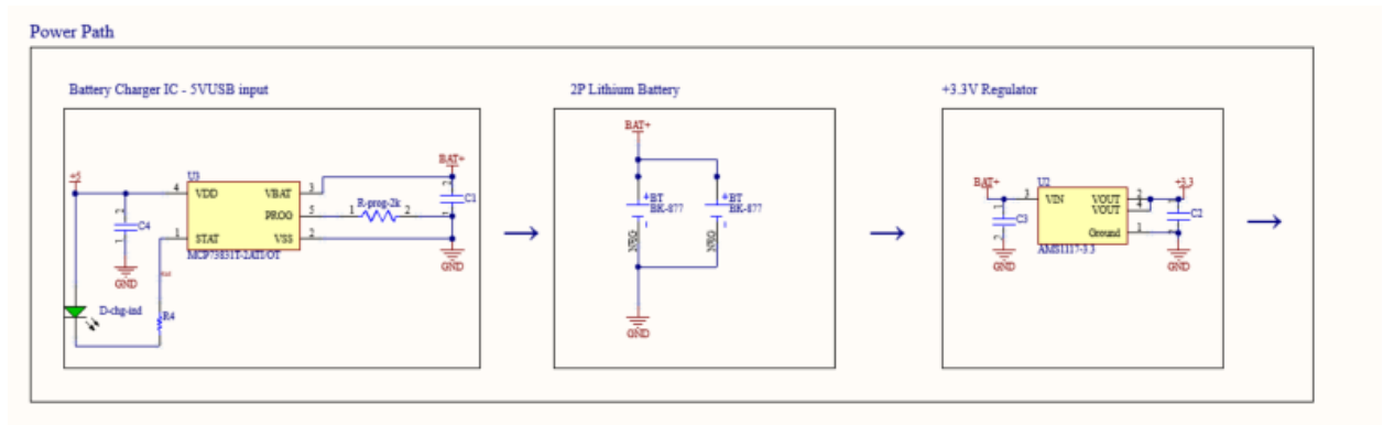
Power path for User input device
