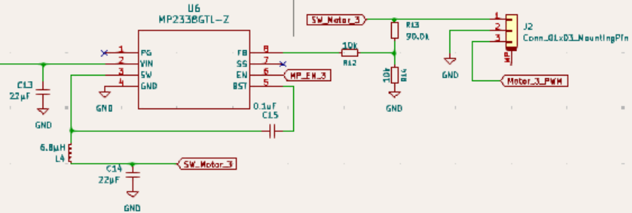
Schematic (2) for the User Output Device
