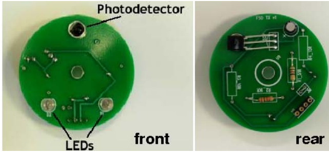
Fig. 3. Transceiver circuit front and rear view.
