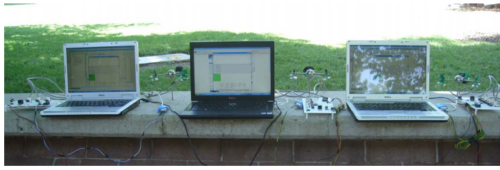
(a) Experiment setup: 3 laptops (collinear placement), each with a 3-transceiver optical antenna.
