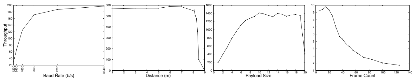
(a) Throughput behavior as baud rate varies. (b) Distance effect on throughput. (c) Payload size effect on throughput. (d) Frame count effect on channel usage.
