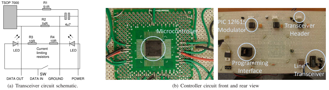
Fig. 2. Schematic of transceiver circuit and picture of controller circuit.
